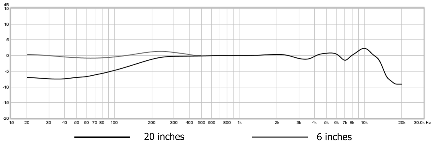
Frequency Response
