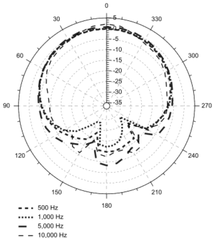
Polar Response
