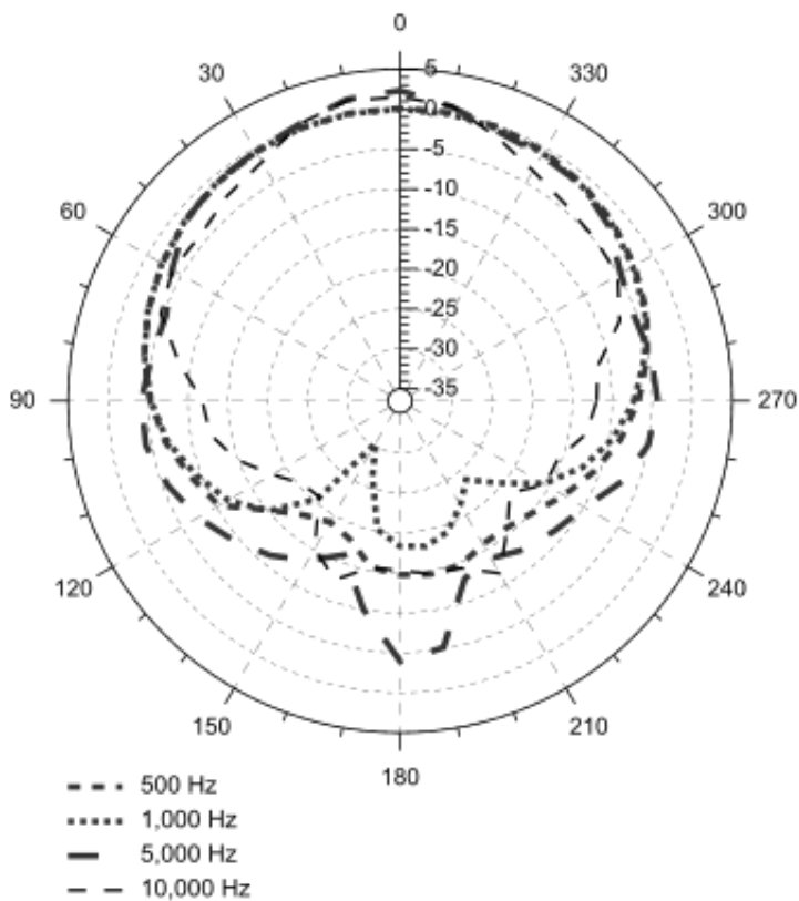
Polar Response
