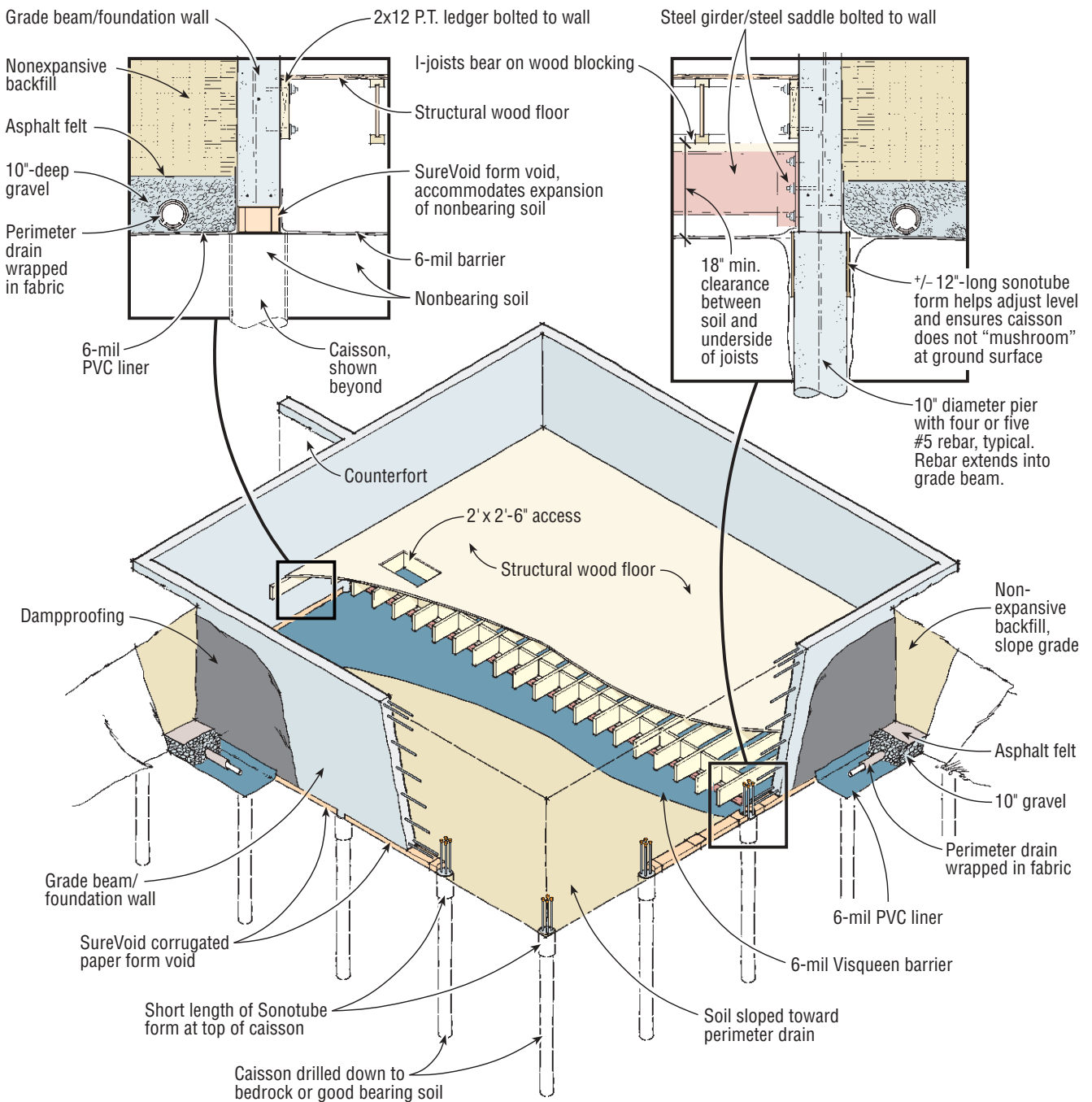
Figure 2. Unlike a conventional poured foundation and continuous strip footing, the heavily reinforced foundation walls of a pier-and-grade-beam foundation are isolated from the underlying soil except where they bear on the caissons, which extend to bedrock or competent bearing soil. Cardboard void forms beneath the nonbearing portions of the walls provide temporary support during the concrete pour but later soften with exposure to soil moisture, creating a space into which the soil can expand without causing damage.
