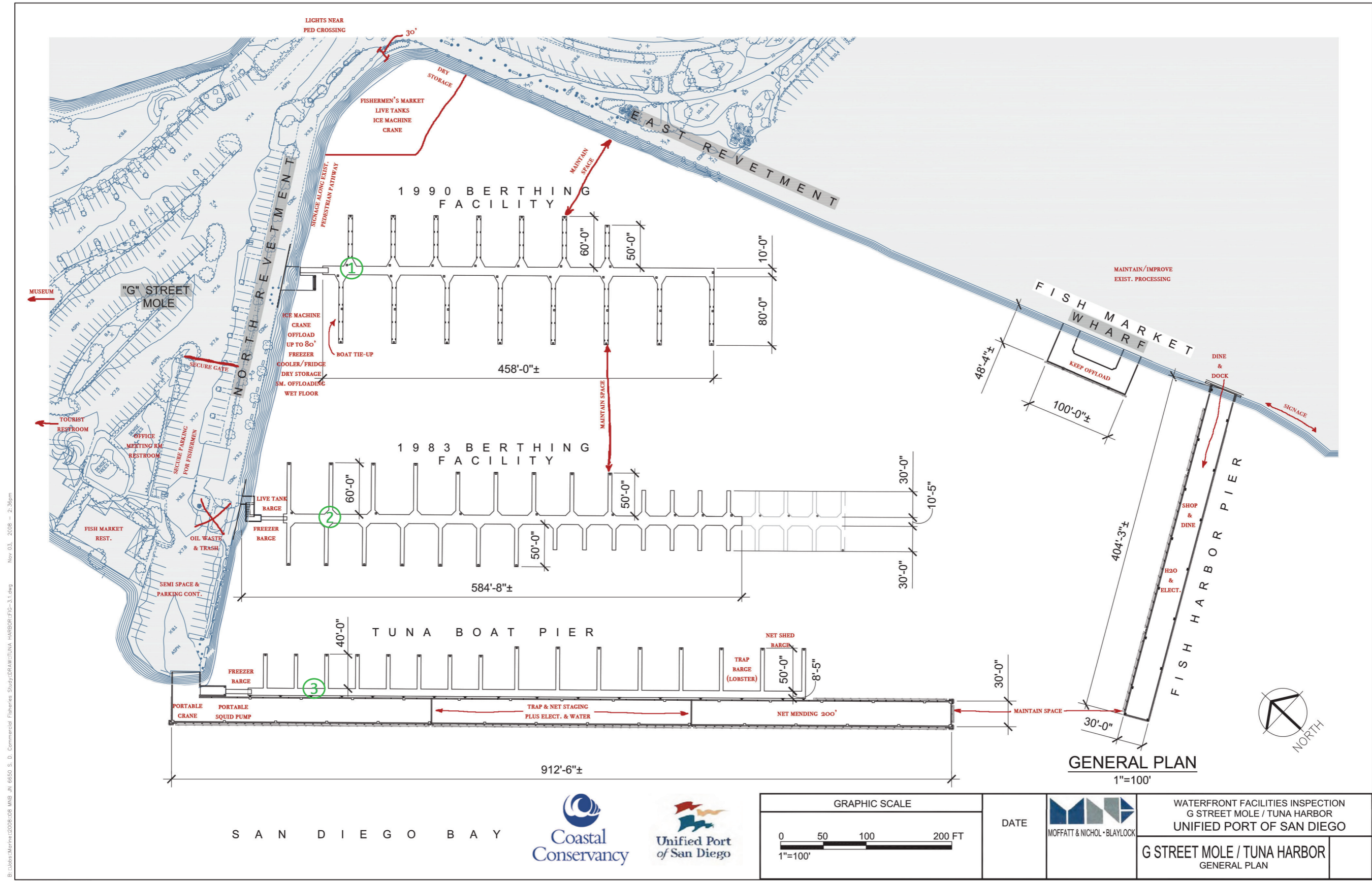
Figure 2.21 Tuna Harbor General Plan
