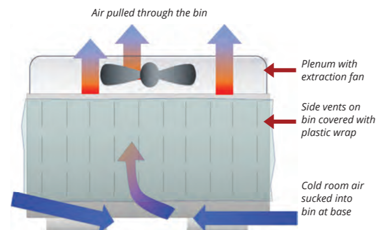
Forced air cooling system for use with bins
