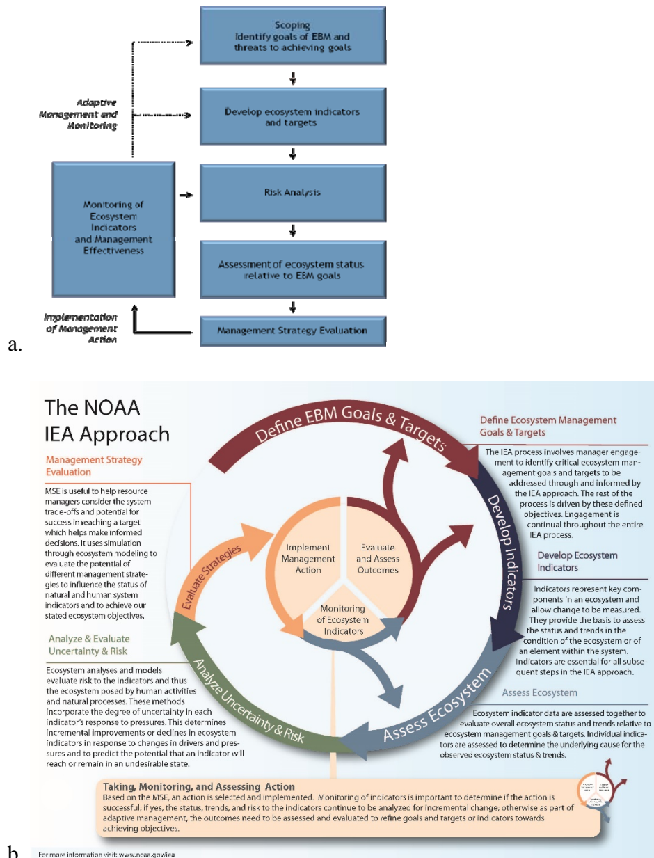
Figure 6. Visualizing IEAs. a. Levin et al (2009) b. Refined IEA representation.
