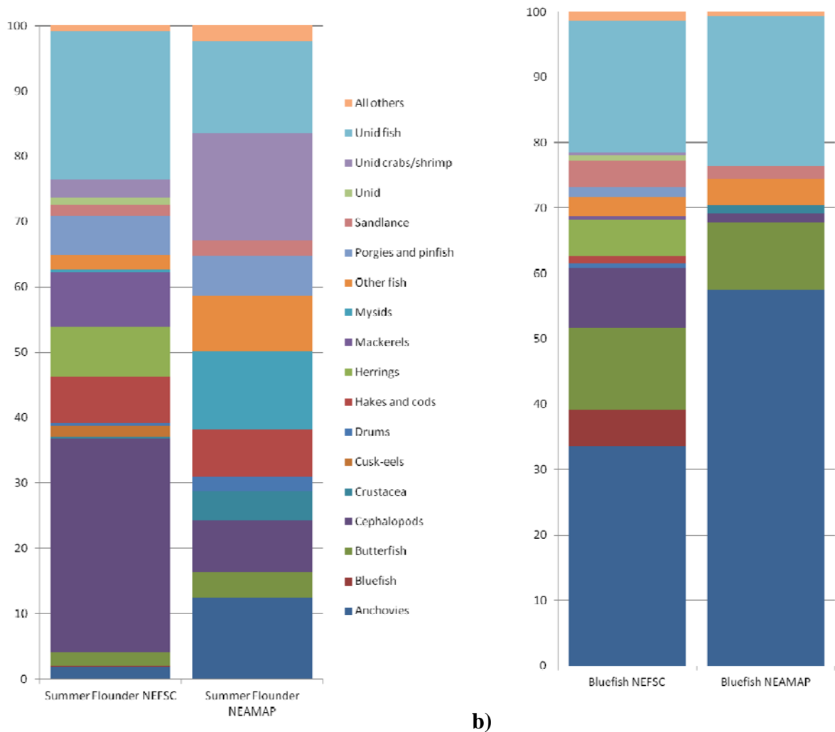
Figure 3. a) Summer flounder diet in the Mid-Atlantic, b) Bluefish diet in the Mid-Atlantic; NEFSC diet database 1963-2012 and NEAMAP database 2006-2012.
