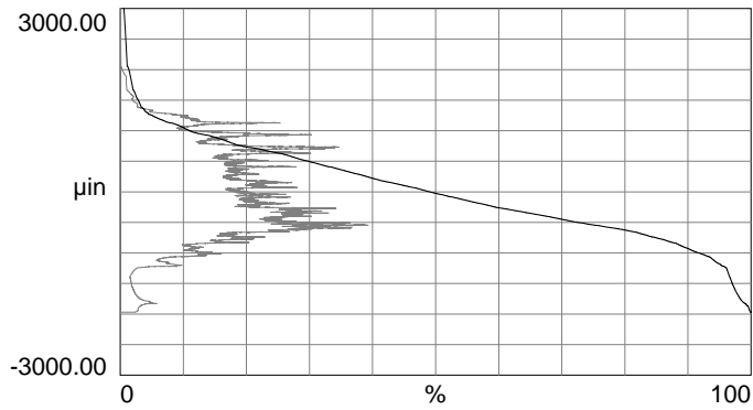
Roughness Profile Bearing Ratio and Amplitude Distribution
