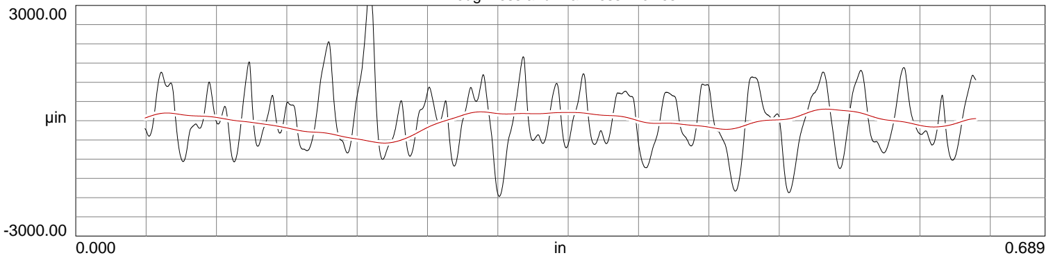
Roughness Profile Bearing Ratio and Amplitude Distribution
