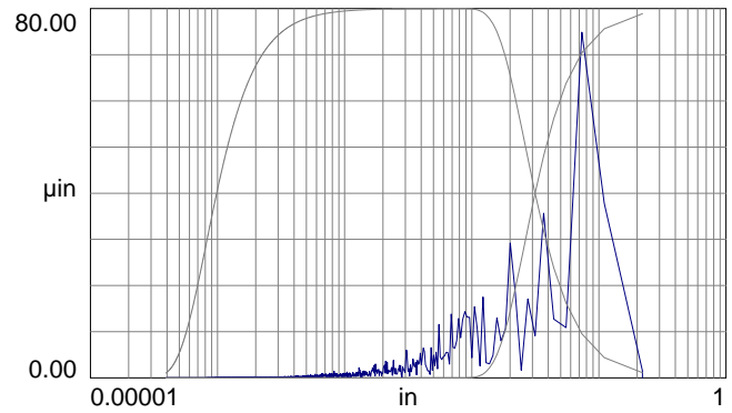
Wavelength Content (Form Suppressed)
