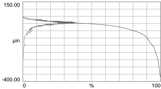
Roughness Profile Bearing Ratio and Amplitude Distribution
