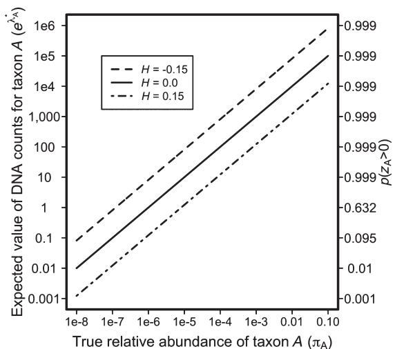
FIG. 3. The expected value of DNA reads for hypothetical taxon A at varying levels of true proportional abundance, \pi_A , for a single PCR primer and 1000000 total DNA reads. The three lines correspond to three possible qualities of match between primer and taxon A . If taxon A has a better than average match with the primer ( H = -0.15 ) it is expected to be observed more frequently than if taxon had an primer match equivalent to the other species in the sample ( H = 0 ) or a below average match ( H = 0.15 ). The right axis shows the probability that the count of taxon A is nonzero. Note that if DNA is infrequent, the probability of detection can be dramatically affected by the primer-template match.
