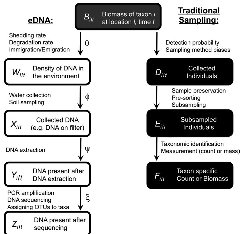
FIG. 1. A schematic illustration of the process of sampling ecological communities using eDNA and traditional sampling methods. Boxes correspond to latent states, while arrows and Greek letters represent processes contributing to the transitions between states. While we present only one eDNA path and one traditional sampling path, recognize that there are many potential variations on the form of this figure depending on the details of a particular protocol.
