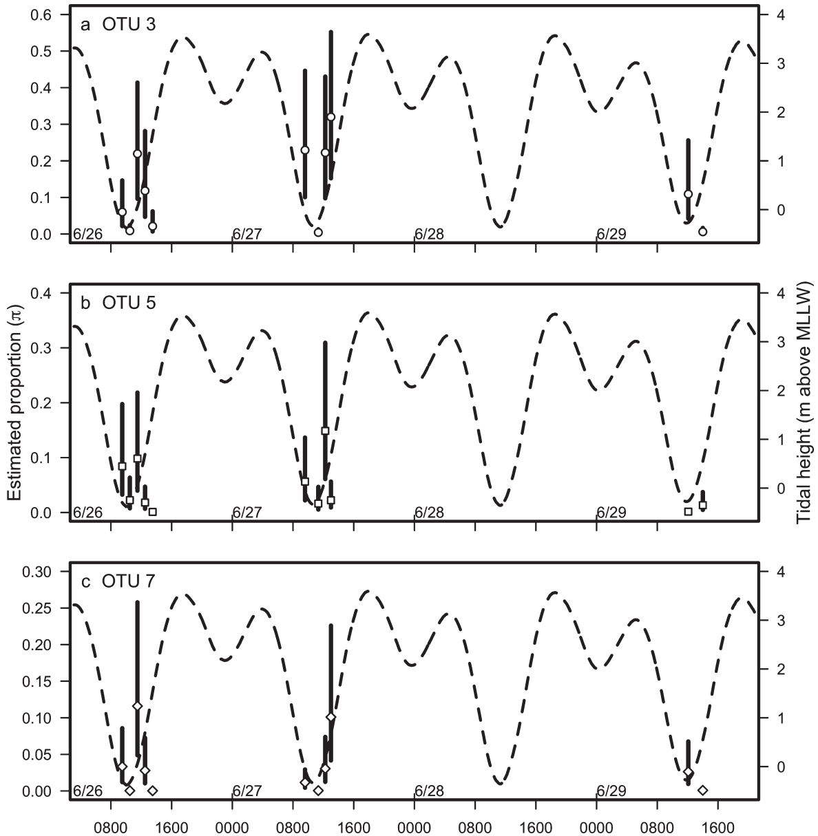
FIG. 5. Time-series for three example OTUs (3, 5, and 7). Median estimated proportion and interquartile range is shown against the tidal height at the sample site (dashed line; height above mean lower low water). Note the left y -axis varies among panels.
