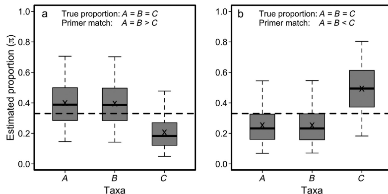
FIG. 2. The effect of primer bias on estimated species composition. In (a), taxa A , B , and C are equally abundant but A and B had identical, average, primer-template matches ( H = 0 ) while C had a below average match to the primer ( H = 0.05 ). In panel (b), taxa A and B are again identical, but C has improved primer match ( H = -0.05 ). The dashed line shows true proportional abundance. Uncertainty bounds represent both uncertainty in the parameter \gamma and approximate uncertainty in the posterior distribution and covariance in the taxon-specific parameters, \beta , derived from our example application (see Supplement S1 for full simulation details). In both panels, boxplots show median, interquartile range, and 95% credible intervals, and x denotes the mean estimate. The horizontal dashed line represents the true proportional abundance. The most important point is that because the estimates are relative proportions that must sum to one, if one taxon has a biased estimate, all of the other taxa's estimates are biased as well.
