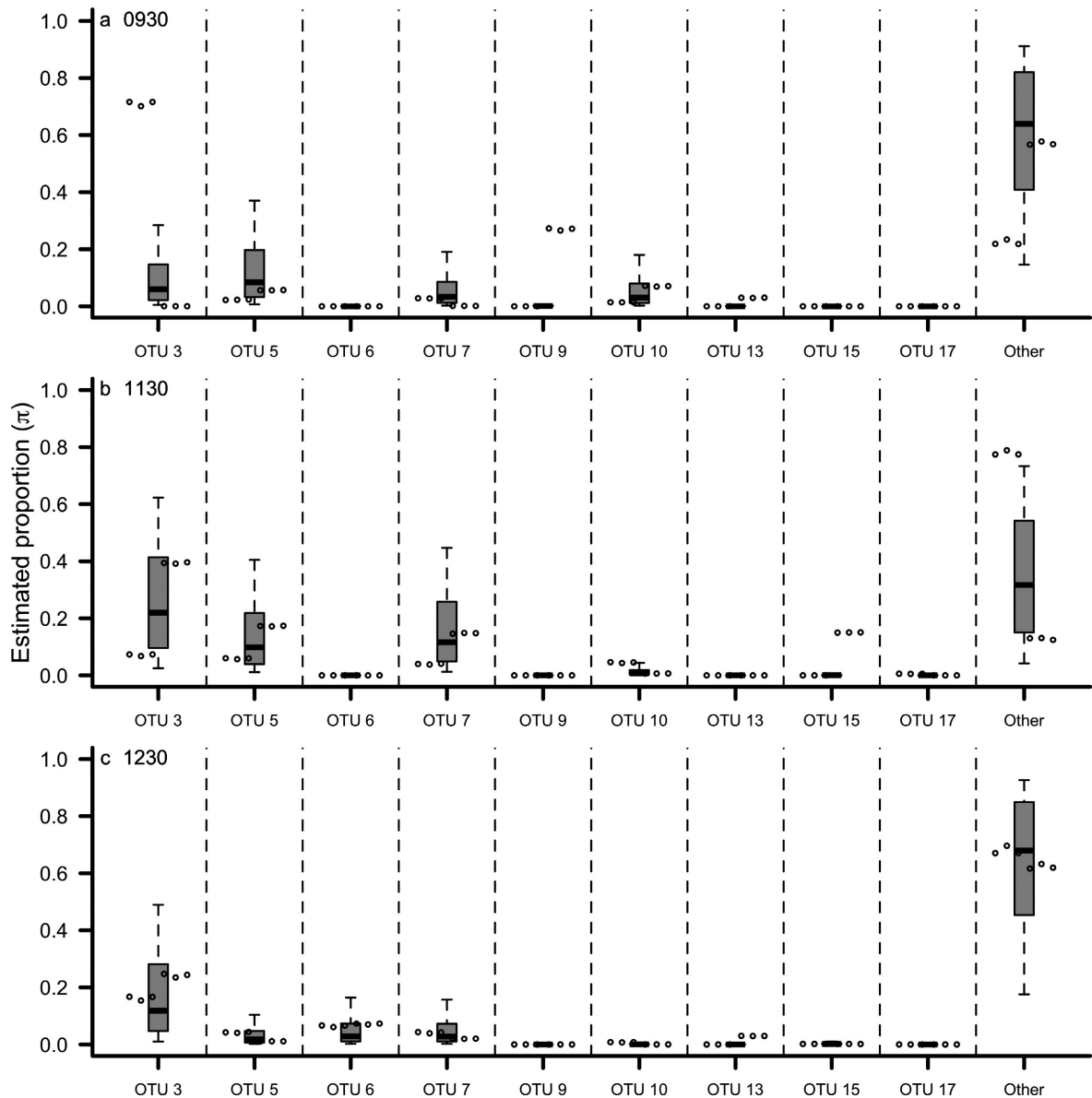
FIG. 4. Estimated proportional contribution for nine unique OTUs and Other for three sampled time periods: (a) 09:30, (b) 11:30, (c) 12:30 on 26 June 2014. Points represent raw counts of DNA sequences for each OTU divided by the total number of DNA reads from individual sequencing runs. Each OTU has six observations, three PCR replicates from each of two PCR primers. Boxplots show the posterior median, interquartile range, and 95% credible interval for each OTU.
