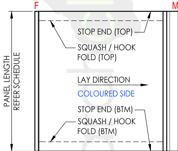
PANEL TYPE (1) - FRONT VIEW
