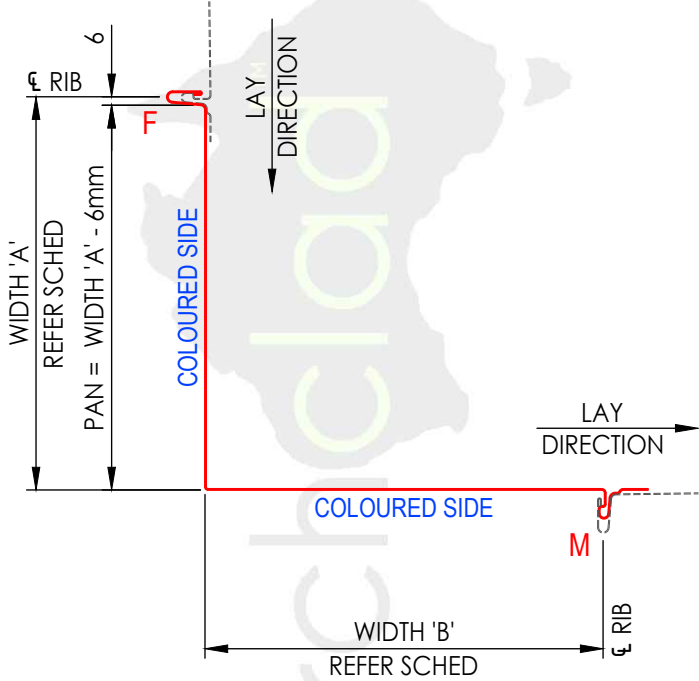
PANEL TYPE (5) - TOP VIEW CLIPTRAY 25 - CORNER
