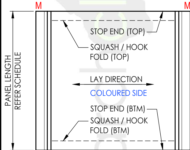
PANEL TYPE (3) - FRONT VIEW
