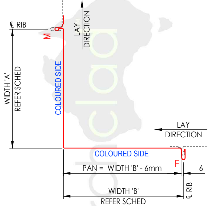
PANEL TYPE (6) - TOP VIEW CLIPTRAY 25 - CORNER
