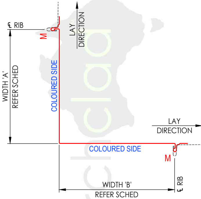
PANEL TYPE (7) - TOP VIEW CLIPTRAY 25 - CORNER
