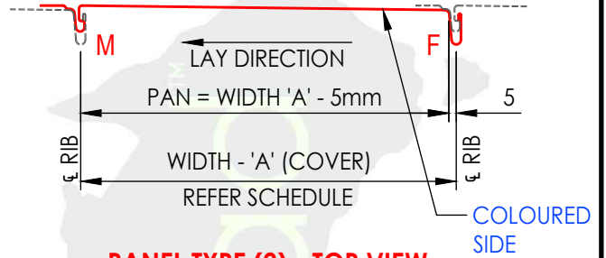
PANEL TYPE (2) - TOP VIEW CLIPTRAY 25 PANEL
