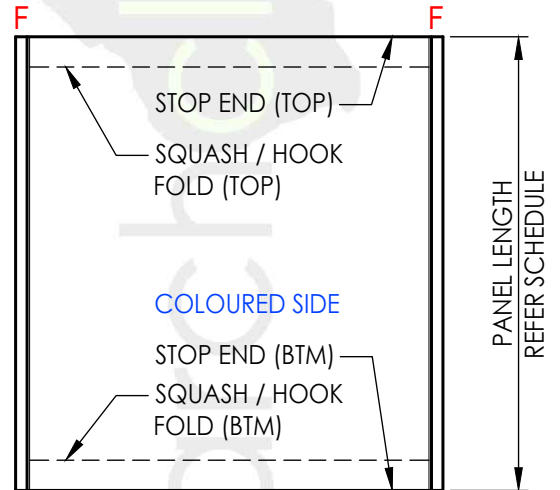
PANEL TYPE (4) - FRONT VIEW
