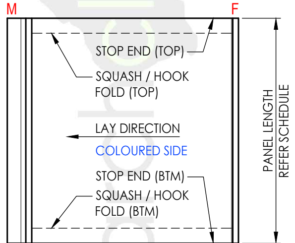
PANEL TYPE (2) - FRONT VIEW
