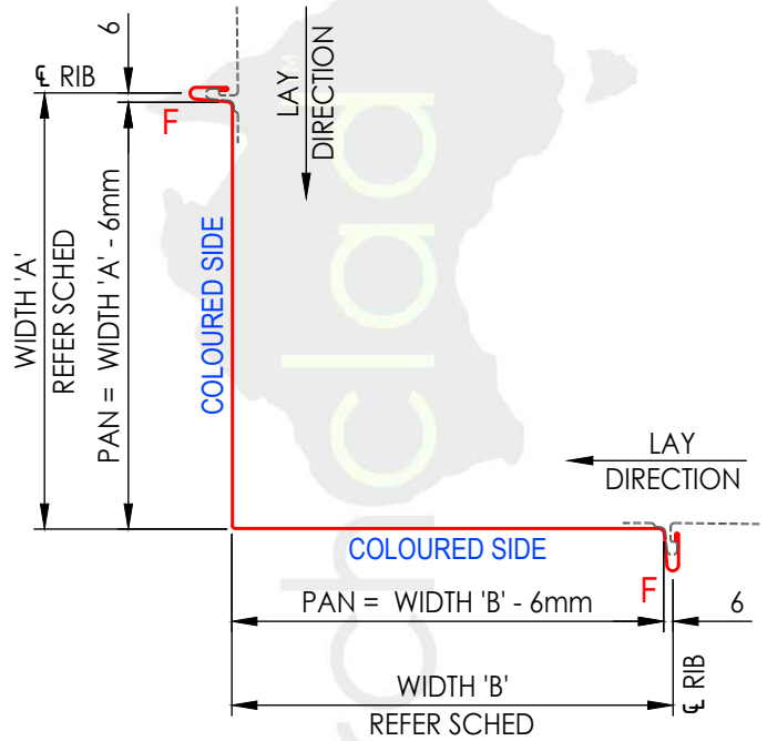
PANEL TYPE (8) - TOP VIEW CLIPTRAY 25 - CORNER
