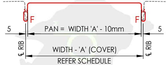
PANEL TYPE (4) - TOP VIEW CLIPTRAY 48 PANEL
