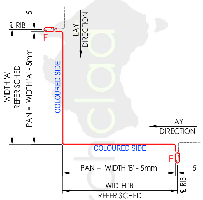
PANEL TYPE (8) - TOP VIEW CLIPTRAY 48 - CORNER
