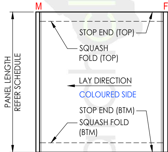
PANEL TYPE (2) - FRONT VIEW
