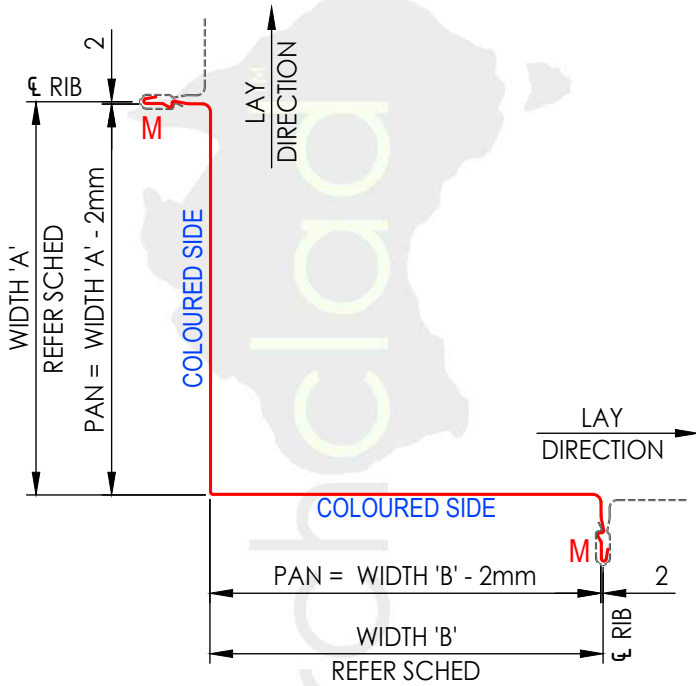
PANEL TYPE (7) - TOP VIEW CLIPTRAY 48 - CORNER
