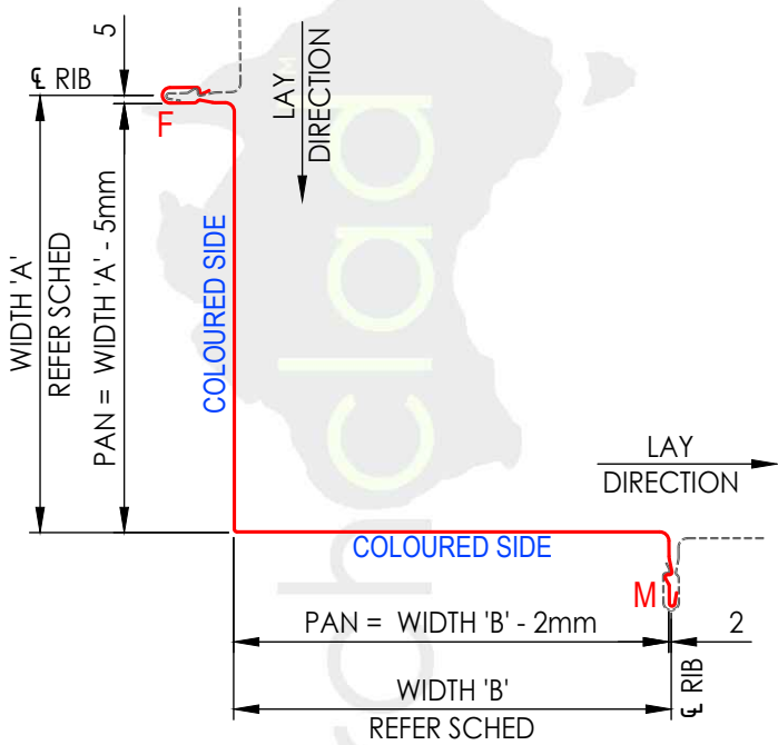
PANEL TYPE (5) - TOP VIEW CLIPTRAY 48 - CORNER
