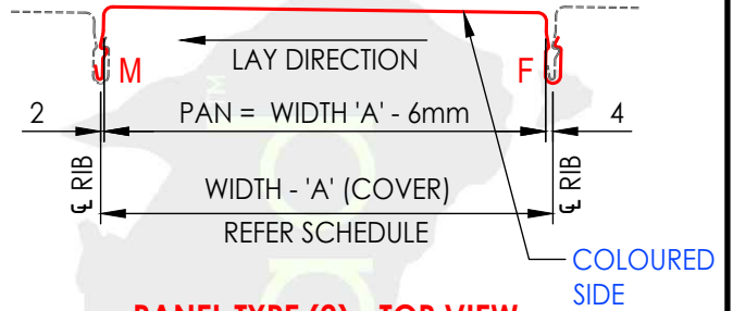
PANEL TYPE (2) - TOP VIEW CLIPTRAY 48 PANEL
