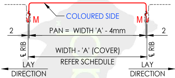
PANEL TYPE (3) - TOP VIEW CLIPTRAY 48 PANEL
