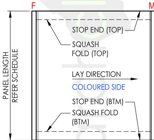
PANEL TYPE (1) - FRONT VIEW
