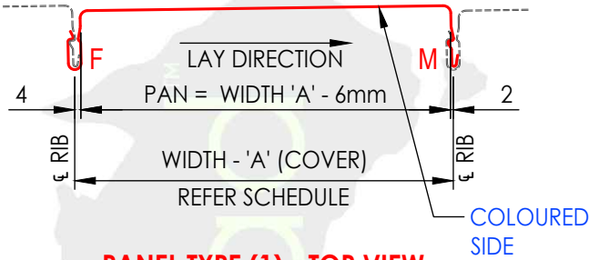
PANEL TYPE (1) - TOP VIEW CLIPTRAY 48 PANEL
