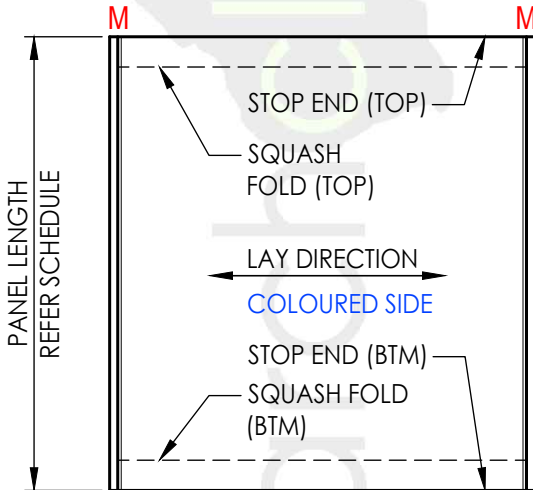
PANEL TYPE (3) - FRONT VIEW
