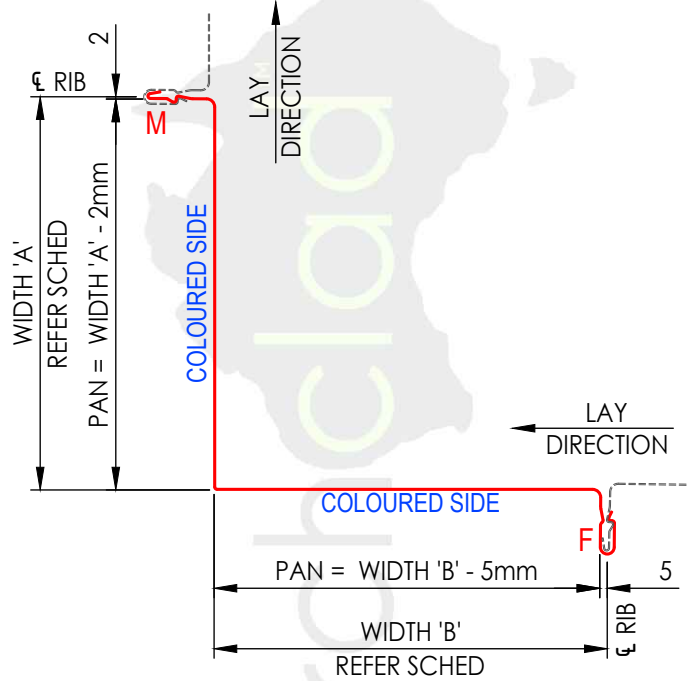
PANEL TYPE (6) - TOP VIEW CLIPTRAY 48 - CORNER
