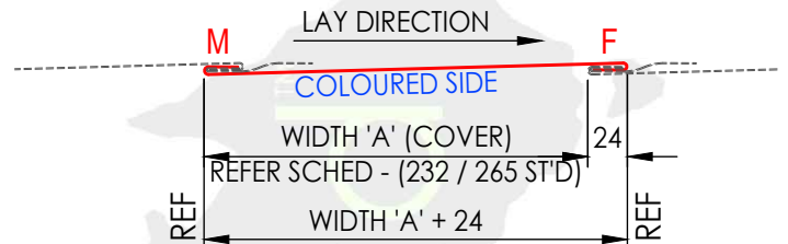
PANEL TYPE (4) - TOP VIEW FLATLOCK PANEL - STANDARD
