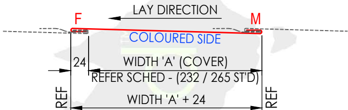
PANEL TYPE (3) - TOP VIEW FLATLOCK PANEL - STANDARD
