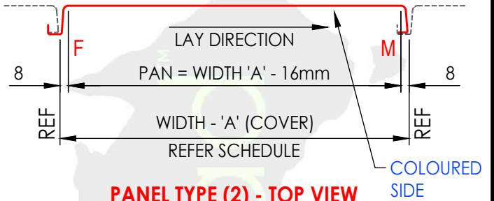
PANEL TYPE (2) - TOP VIEW STANDING SEAM PANEL SINGLE LOCK
