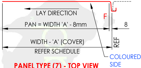
PANEL TYPE (7) - TOP VIEW STANDING SEAM - END PANEL SINGLE LOCK
