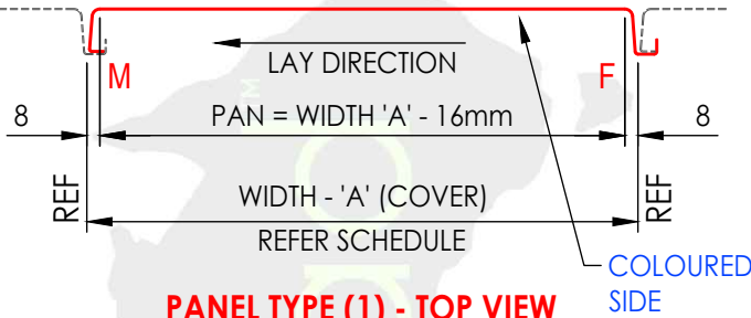
PANEL TYPE (1) - TOP VIEW STANDING SEAM PANEL SINGLE LOCK
