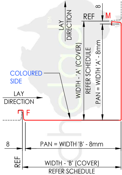
PANEL TYPE (14) - TOP VIEW STANDING SEAM - INTERNAL CORNER PANEL SINGLE LOCK
