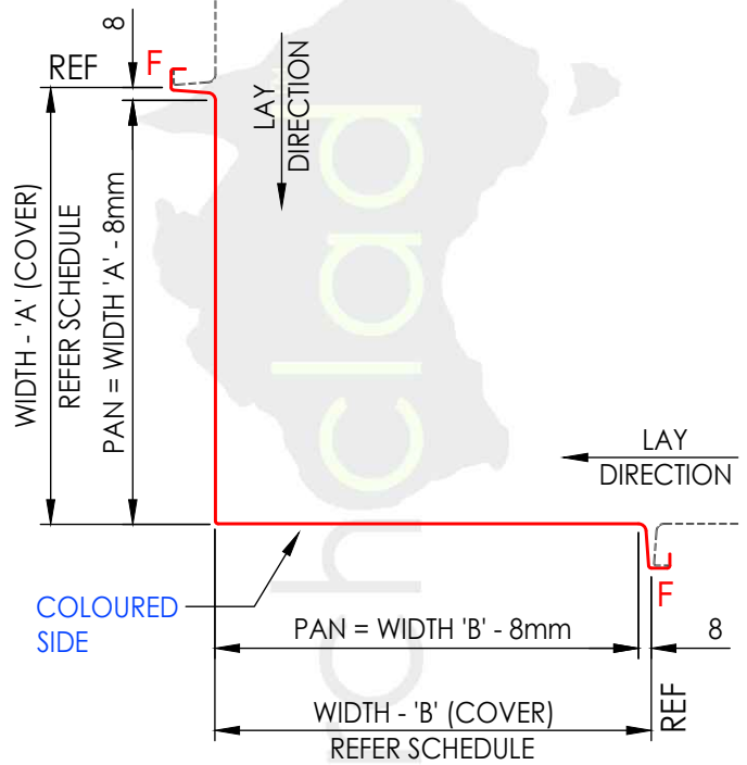
PANEL TYPE (12) - TOP VIEW STANDING SEAM - END CORNER PANEL SINGLE LOCK
