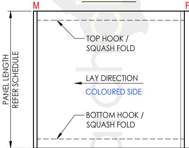
PANEL TYPE (1) - FRONT VIEW
