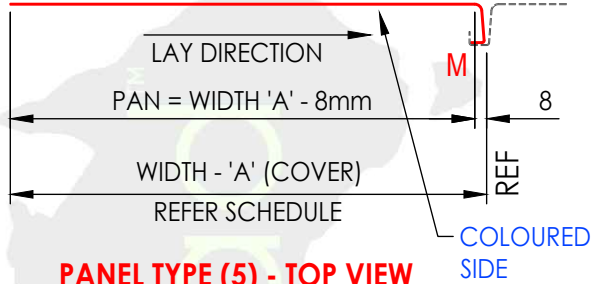
PANEL TYPE (5) - TOP VIEW STANDING SEAM - STARTER PANEL SINGLE LOCK
