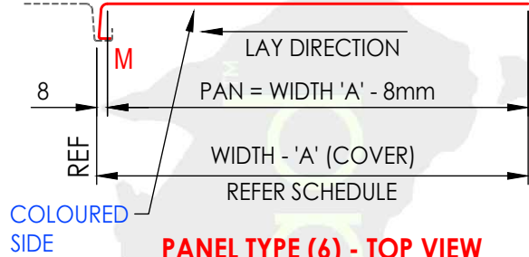
PANEL TYPE (6) - TOP VIEW STANDING SEAM - STARTER PANEL SINGLE LOCK
