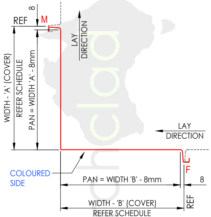
PANEL TYPE (10) - TOP VIEW STANDING SEAM - CORNER PANEL SINGLE LOCK
