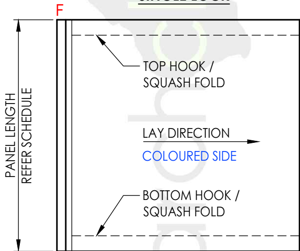
PANEL TYPE (8) - FRONT VIEW
