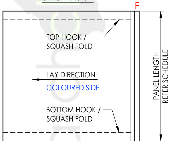
PANEL TYPE (7) - FRONT VIEW
