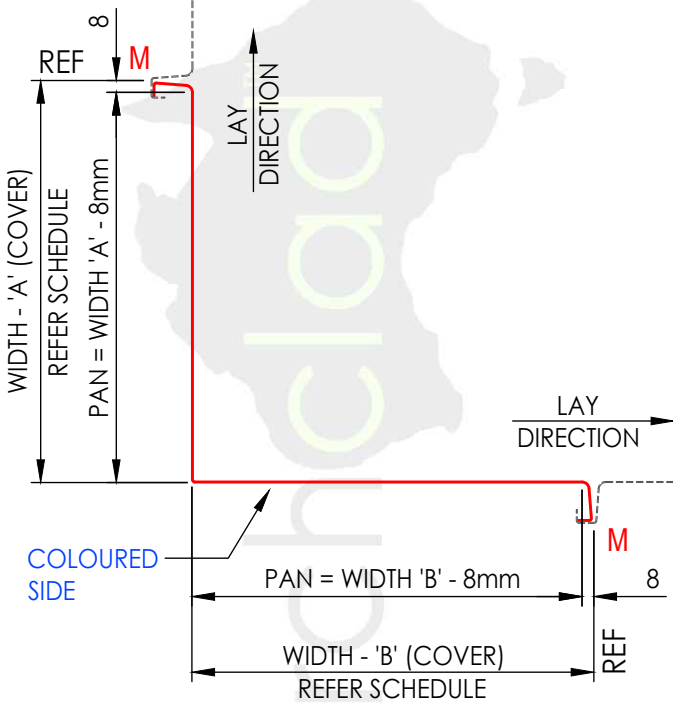
PANEL TYPE (11) - TOP VIEW STANDING SEAM - STARTER CORNER PANEL SINGLE LOCK
