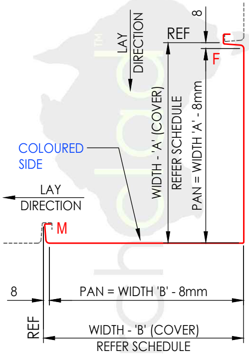
PANEL TYPE (13) - TOP VIEW STANDING SEAM - INTERNAL CORNER PANEL SINGLE LOCK
