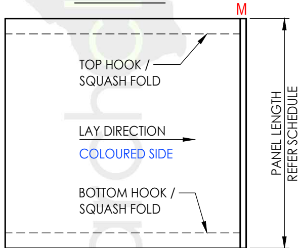
PANEL TYPE (5) - FRONT VIEW
