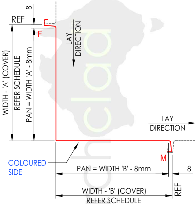
PANEL TYPE (9) - TOP VIEW STANDING SEAM - CORNER PANEL SINGLE LOCK
