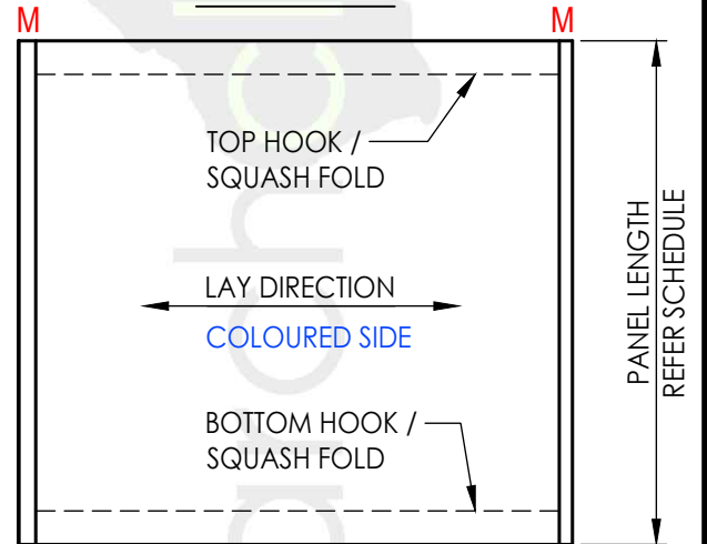
PANEL TYPE (4) - FRONT VIEW
