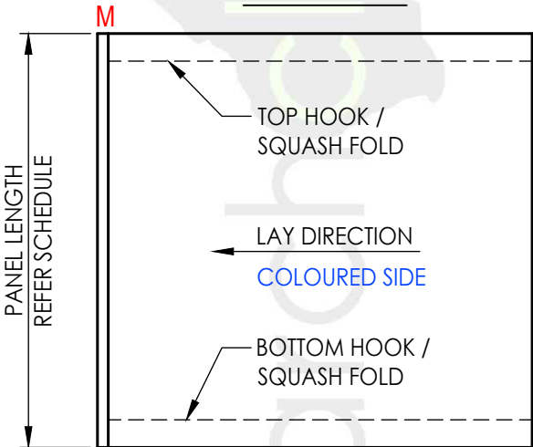
PANEL TYPE (6) - FRONT VIEW
