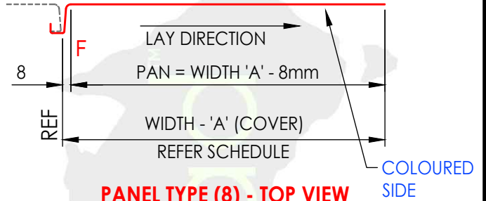
PANEL TYPE (8) - TOP VIEW STANDING SEAM - END PANEL SINGLE LOCK
