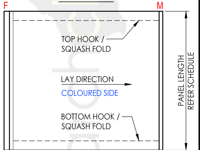
PANEL TYPE (2) - FRONT VIEW
