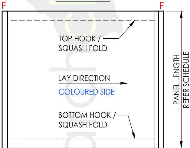
PANEL TYPE (3) - FRONT VIEW
