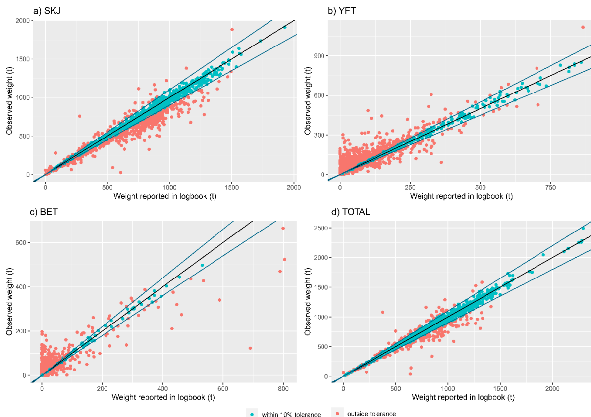
Figure 12: Comparisons of weights recorded in logsheets and observer reports for individual target tuna species and total weight at the TRIP level in the purse seine fishery, 2017-2019. (n=1630; Black lines show a 1:1 relationship between logsheet and observer estimates. Red data points are outside of the 10% tolerance level.)
