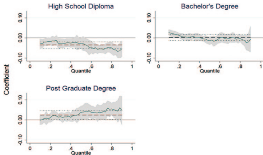
Figure 7. All Opinions. Quantile regression results (solid line) with 90 percent confidence interval (shaded gray), OLS result (dashed), and OLS 90 percent confidence interval (dotted).
