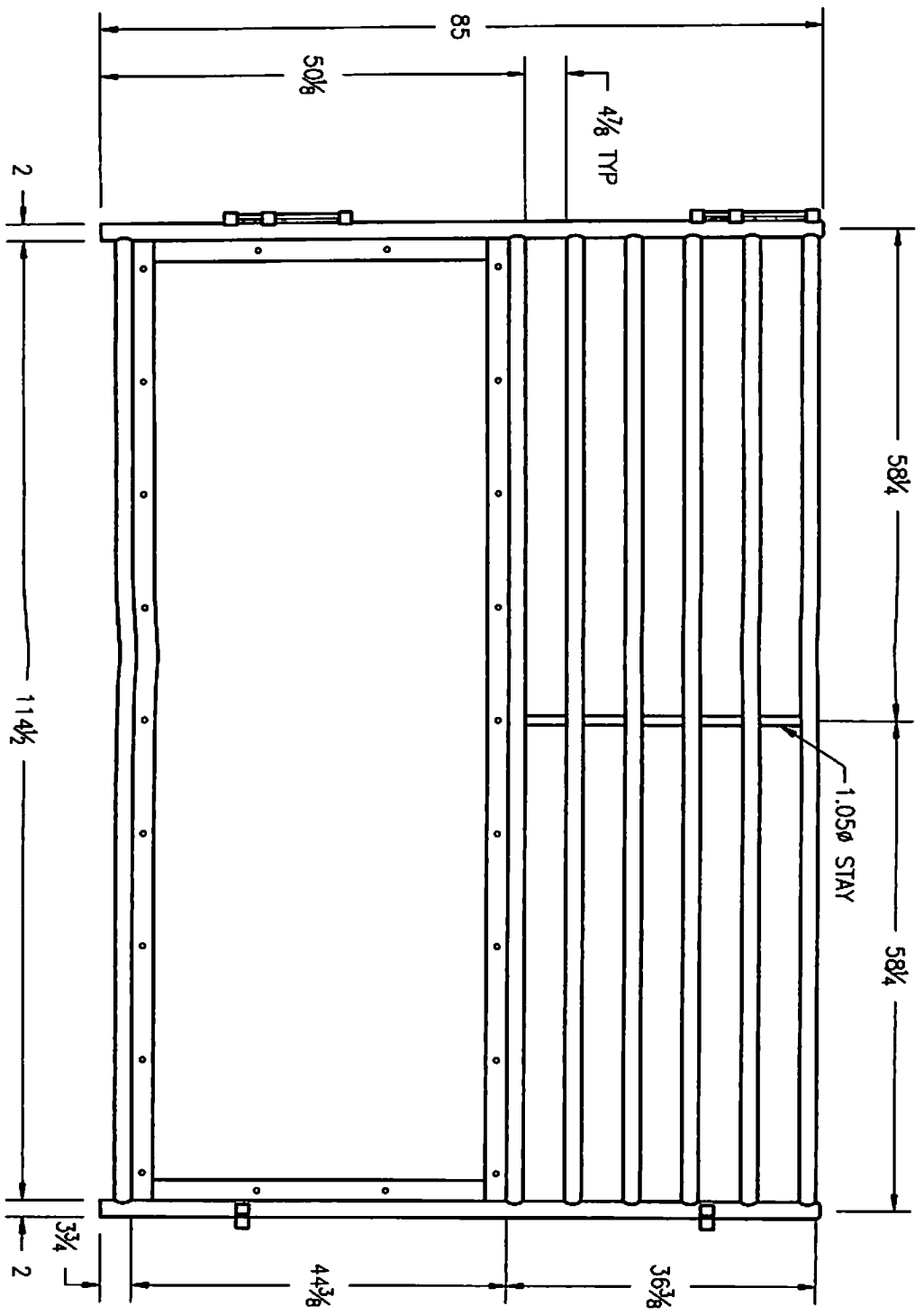
FRONT VIEW
