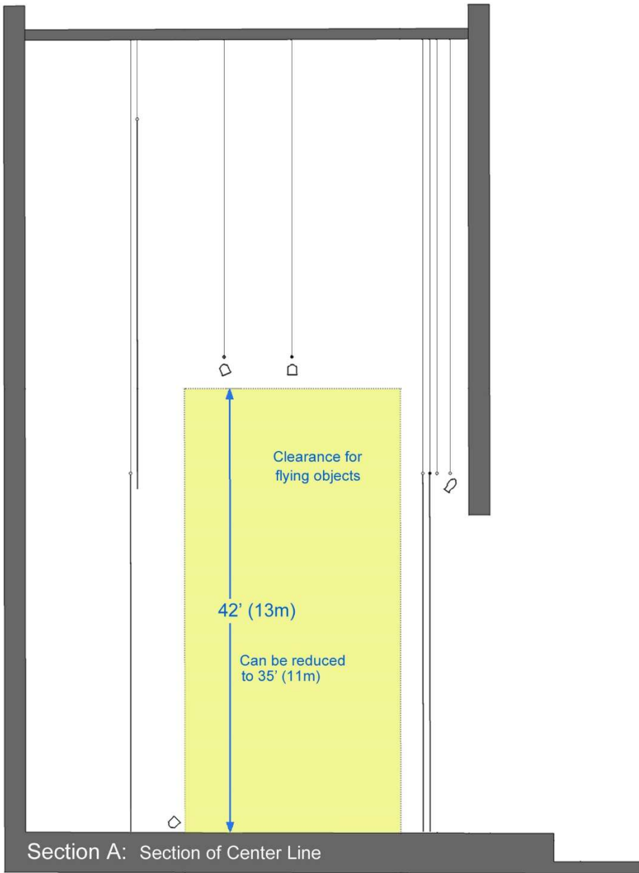
AIR PLAY Sections Scale 1:150 TL July 2016
