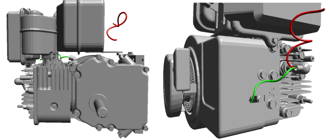
Fig. 6. Two industrial cases of disassembling for a free-flying cable (left) and a fixed base cable (right). The cable has to get out from a highly constrained start configuration (in green) to a low constrained configuration (in red).
