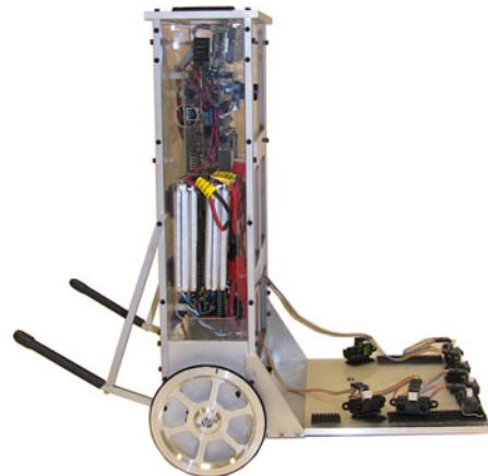
Fig. 6. Differential-drive robot used for experimental validation.
