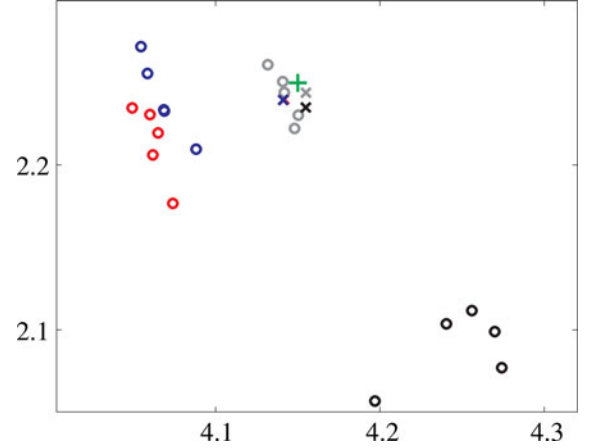
Fig. 9. Ending position for each run. Green “+” for goal position, “x” for expected ending position under zero odometry drift, “o” for actual ending positions. Red, gray, blue, and black plots correspond to 10.16-, 10.48-, 12.7-, and 15.24-cm wheels. Units are in meters (note the zoomed scale).
