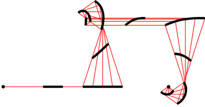
Fig. 2. Ensemble with \epsilon \in [0.8, 1.2] moving a unit distance in the x direction achieving fourth-order error in |\epsilon - 1| , which corresponds to a maximum error bound of 0.2^3 = 0.008 . Thin red lines show the path followed for particular values of \epsilon . The actual robot follows only one of these paths. Thick black lines show the entire ensemble at instants of time.
