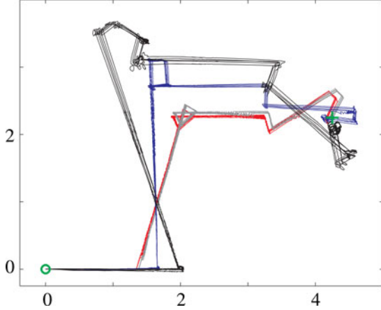
Fig. 8. Ground truth data gathered from the camera system. Five runs for each wheel set are shown. Loops at the corners are artifacts from the camera system. Red, gray, blue, and black plots correspond to 10.16-, 10.48-, 12.7-, and 15.24-cm wheels, respectively. Units are in meters.
