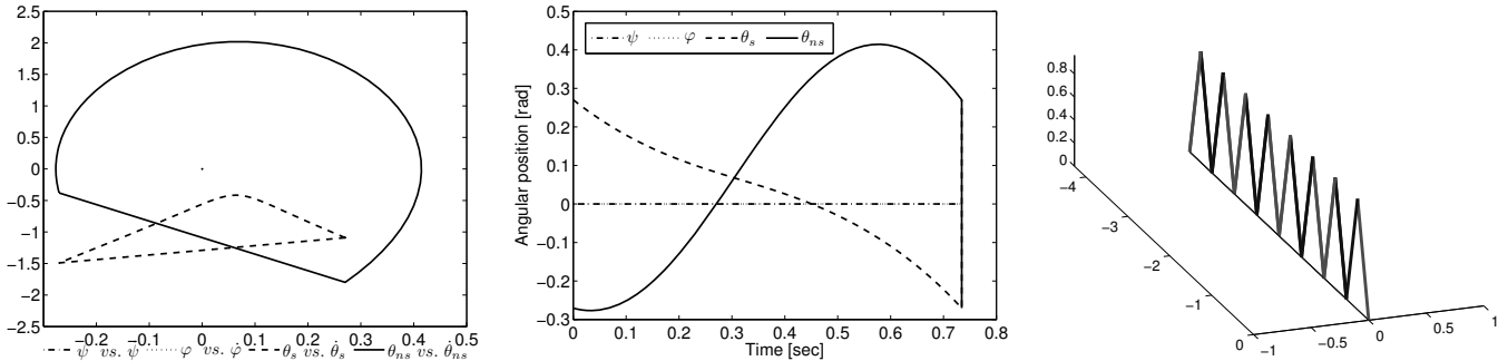
Fig. 3. Straight-ahead 1-step gait: phase portrait (left), coordinate trajectories (center), and multi-step visualization (right). The phase portrait shows planar slices of \mathcal{O}_{4D}^s by plotting angular positions against angular velocities, which we use to illustrate 1-step periodicity in phase space.
