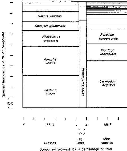
FIG. 3. A model of the division of niche-space along two principle dimensions in grassland. The model is applied to data from plot 3 (unfertilized) of the PGE, 1948. Only the principle species in each component are named.
