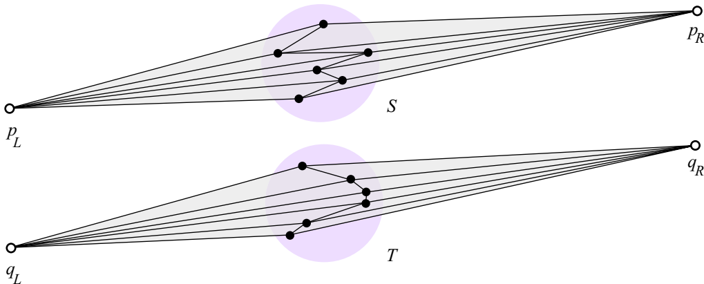
FIGURE 2. Example of sufficiency of two exterior Steiner points.
