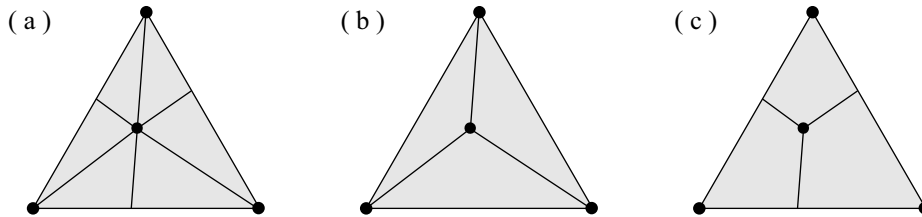
FIGURE 4. (a) Subdivision, (b) trisection, and (c) Y-section of a triangle.
