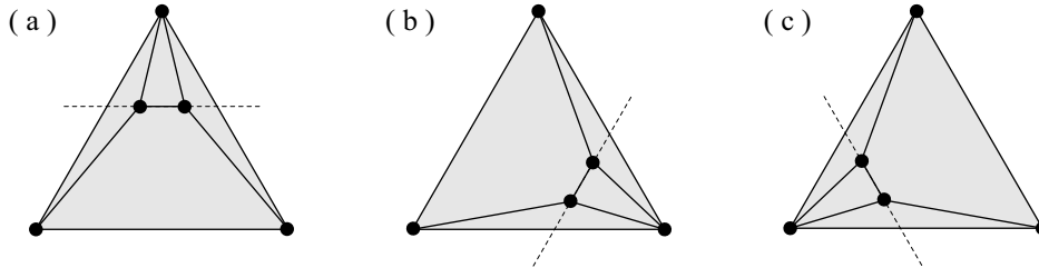
FIGURE 6. Three point sets in Steiner point triangles and their forced edges.
