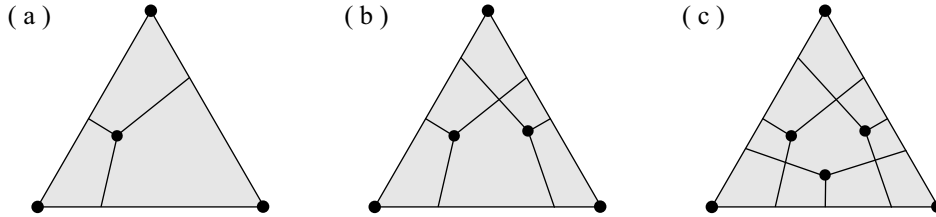
FIGURE 5. The Y-sections of (a) one, (b) two and (c) three points.
