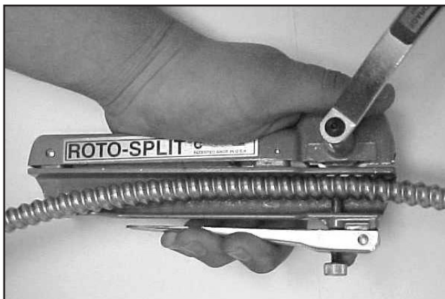
Figure 6.3—Roto Split (courtesy Alflex Cable)
