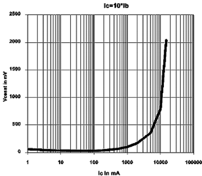
Fig 2: Collector Current Continuous vs Collector Emitter Saturation
