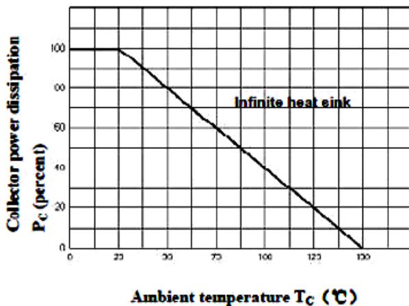
Fig 3: Collector Power Dissipation vs ambient Temp
