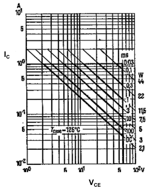
Fig 4: Permissible Operating Range
