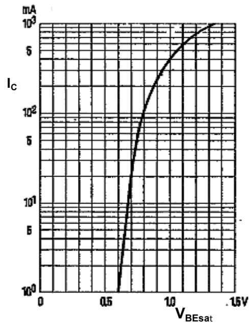
Fig 8: Base-Emitter Saturation Voltage
