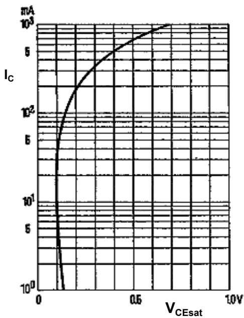
Fig 6: Collector-Emitter Saturation Voltage
