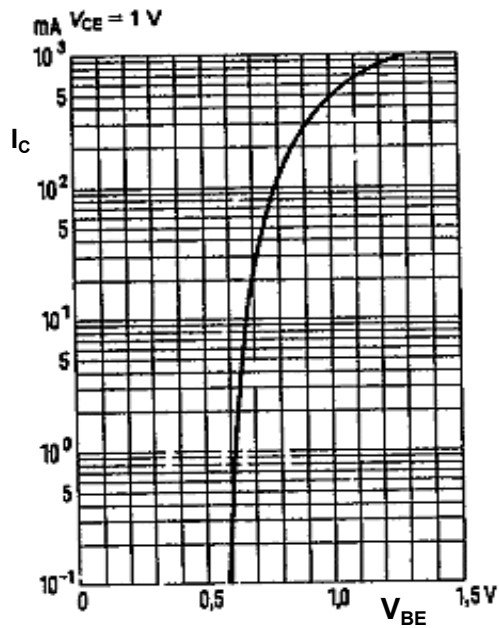
Fig 9: Collector Current I_C = f(V_{BE})
