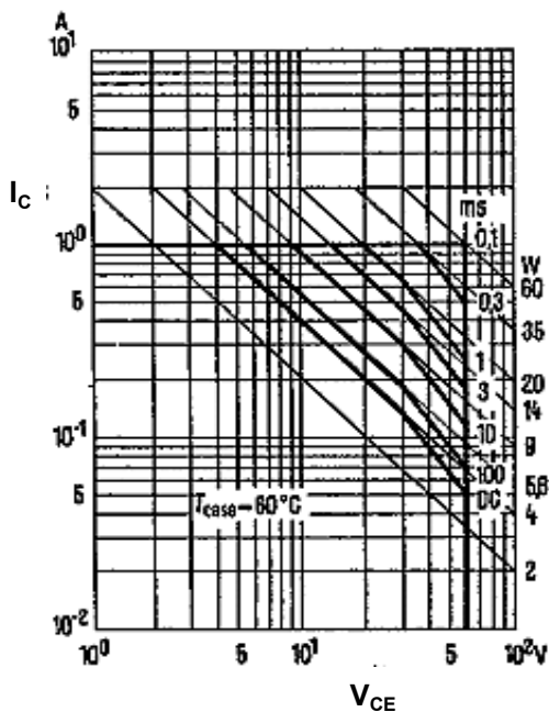
Fig 2: Permissible Operating Range
