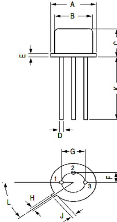
TO-39 Metal Can Package
