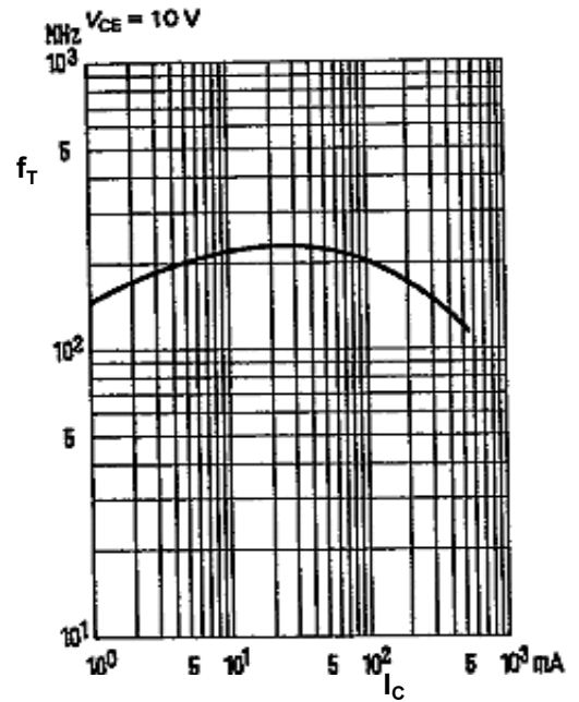
Fig 10: Transition frequency f_T = f(I_C)
