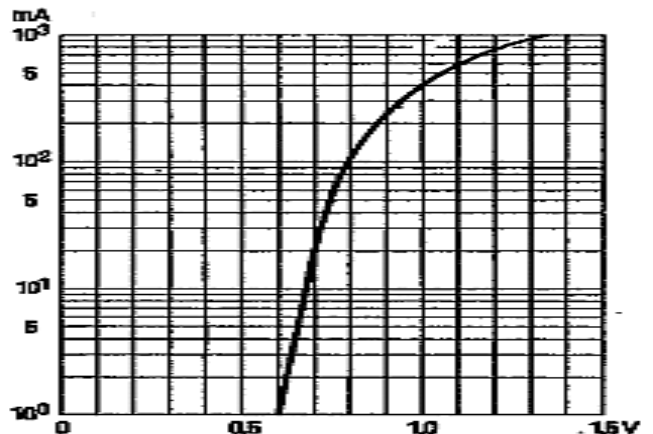
Fig 8: Base-Emitter Saturation Voltage
