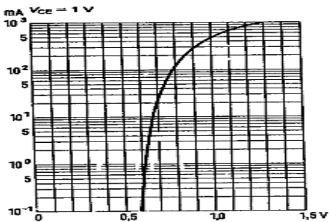
Fig 9: Collector Current I_C = f(V_{BE})
