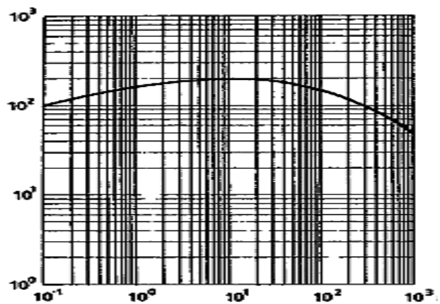
Fig 3: DC Current Gain h_{FE} = f(I_C) V_{CE} = 5V ; T_{amb} = \text{Parameter}
