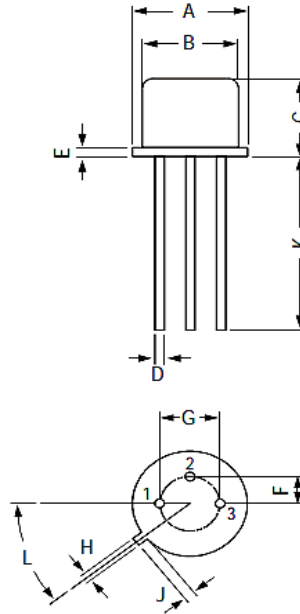
TO-39 Metal Can Package
