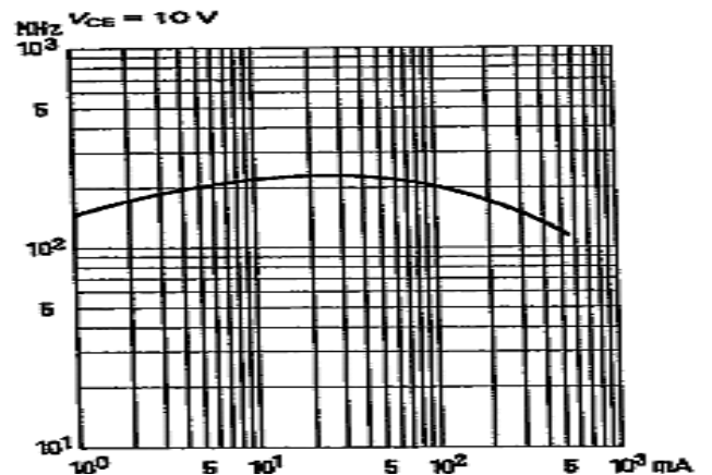
Fig 10: Transition frequency f_T = f(I_C)
