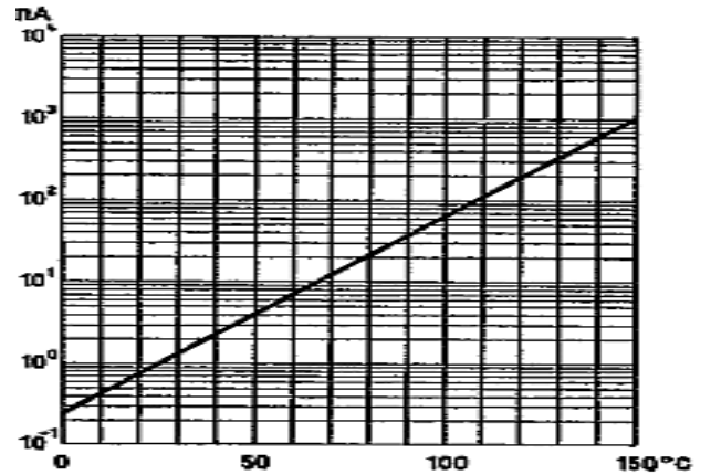
Fig 7: Collector Cutoff Current Versus Temperature I_{CBO} = f(T_{amb}) nA - V_{CE} = 60V
