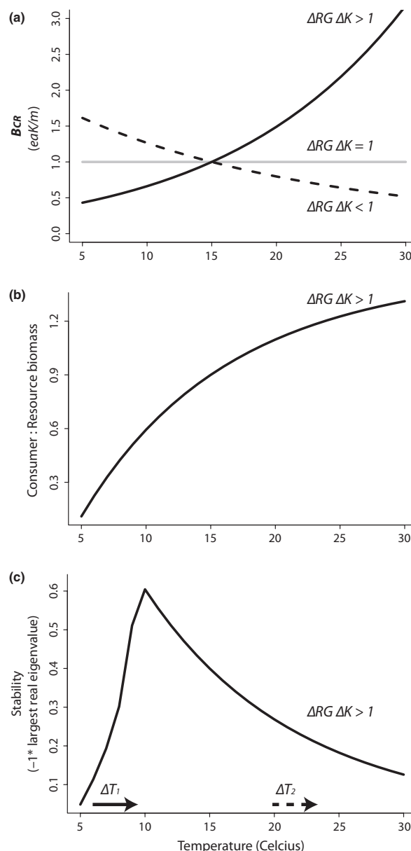
Figure 3 The effect of temperature on B_{CR} , equilibrium C:R biomass ratio, and stability. As temperature increases B_{CR} will increase if an asymmetry causes an increase in resource biomass accumulation or consumer growth (black line), and will decrease in the opposite scenario (dashed line; a). When raising temperature increases B_{CR} , consumers become more abundant relative to resources at higher temperatures (b). Increasing B_{CR} with temperature causes the interaction to become more stable when B_{CR} is initially low (solid arrow) but then destabilises over most of the temperature range (dashed arrow; c). Different stability responses depend on the starting conditions, as even identical changes in temperature produce different stability responses ( \Delta T_1 = \Delta T_2 ; c). For the numerical solutions in panels b and c, K varied with temperature, with E_b=0.32 , E_s=0.9 and K(15 \text{ Celcius})=100 . Other parameters were held constant ( a=0.1 , e=0.15 , m=0.6 , r=2 ).
