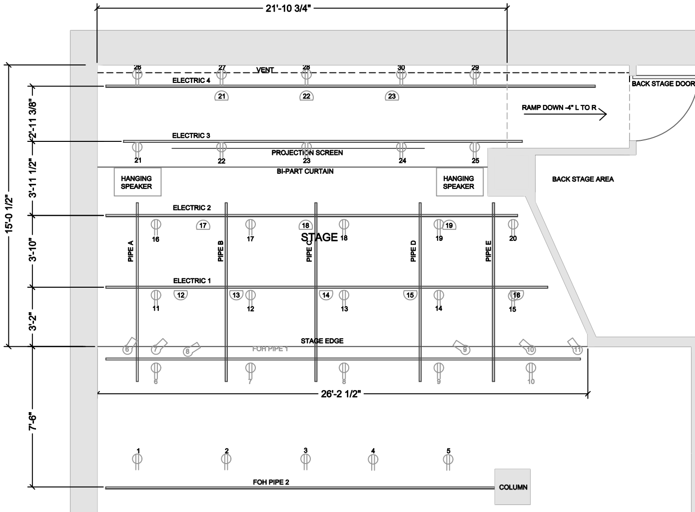
LIGHTING GROUND PLAN N.T.S.
