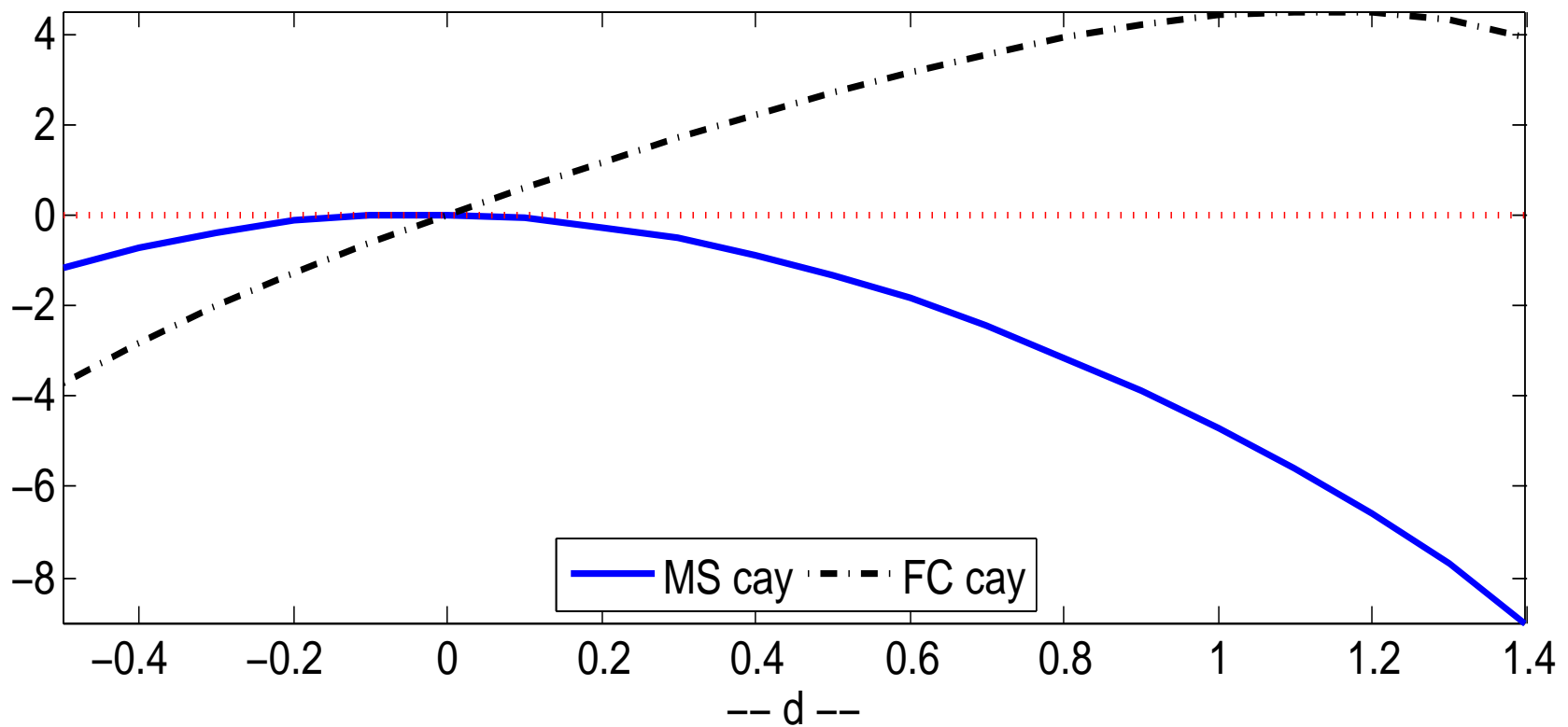
Figure 4: Low frequency log likelihood values for (1 - L)^d \text{cay}_t . The sample is quarterly and spans the period 1952:Q1 to 2013:Q3.
