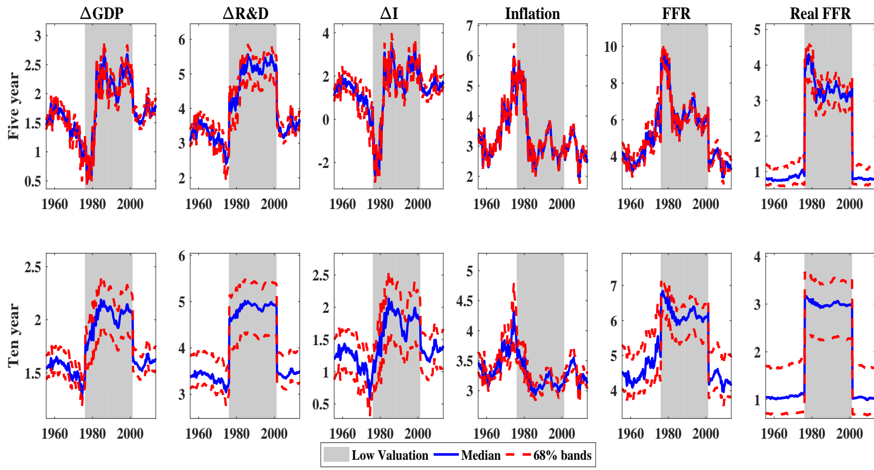
Figure 5: Conditional expectations from baseline MS-VAR. The figure reports the conditional expectations based on the baseline MS-VAR at different horizons taking into account the possibility of regime changes. The sample spans 1955:Q3 to 2013:Q3.
