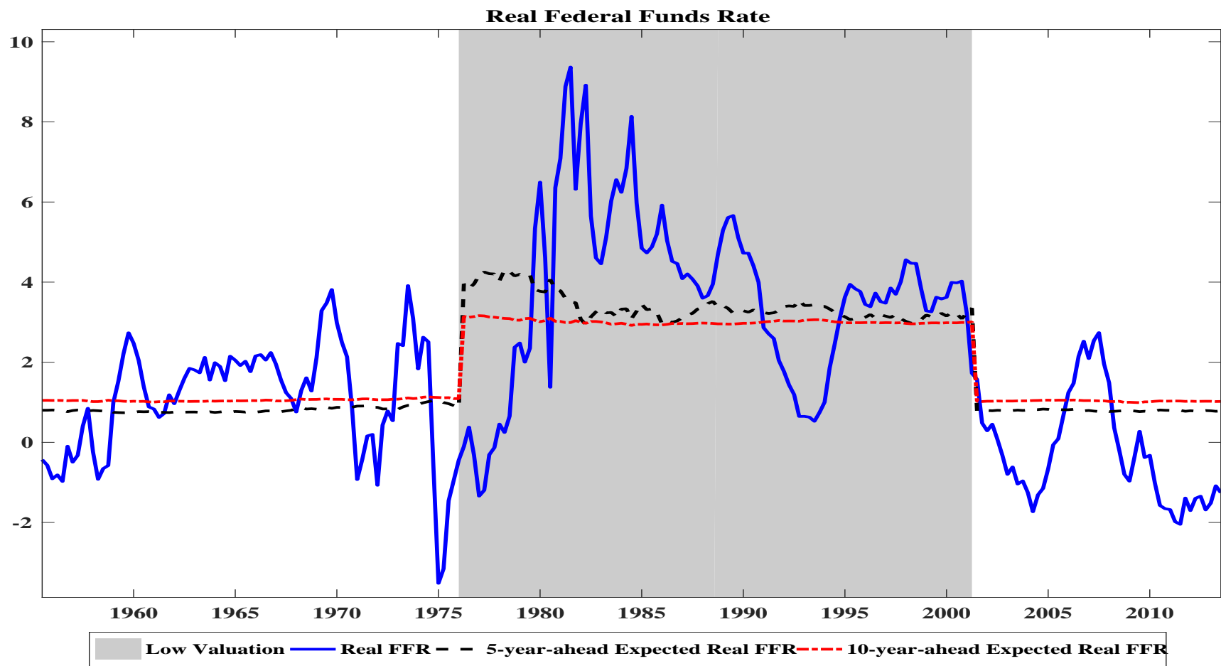
Figure 7: Real Federal Funds Rate. The figure reports the evolution of the Real FFR over time together with the 5-year-ahead and 10-year-ahead expectations as implied by the baseline MS-VAR. Expectations are computed taking into account the possibility of regime changes. The sample spans 1955:Q3 to 2013:Q3.
