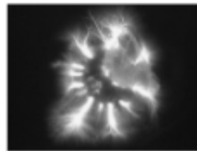
Rose Quartz
