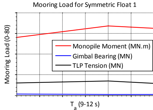
FIGURE 8: PREDICTED ORCAFLEX LOADS FOR SURVIVAL CONDITIONS OF DIFFERENT WAVE PERIODS
