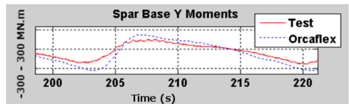
FIGURE 4: EXAMPLE OF ORCAFLEX MODELING OF SPAR LOADS
