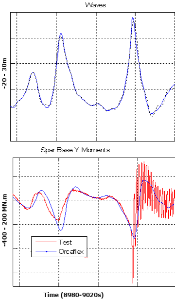
FIGURE 7: EXAMPLE COMPARISON OF ORCAFLEX SIMULATION AND WAVE TANK MEASUREMENTS DURING A SLAM EVENT. TOP: SEA SURFACE ELEVATION. BOTTOM: MOMENT AT SPAR BASE.
