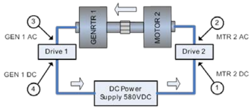
FIGURE 13: SETUP FOR BACK-TO-BACK TESTING OF GENERATOR-DRIVE
