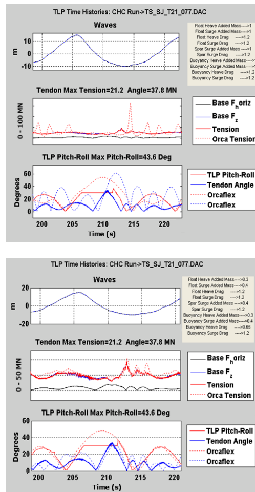
FIGURE 6: EXAMPLE COMPARISON OF CONVENTIONAL (TOP) AND TUNED HYDRODYNAMIC COEFFICIENTS (BOTTOM) USED IN ORCAFLEX (DASHED) TO SIMULATE LOADS. TANK MEASUREMENTS (SOLID) SHOWN FOR COMPARISON. ONLY SHORT PERIOD OF TOTAL TEST TIME IS SHOWN.
