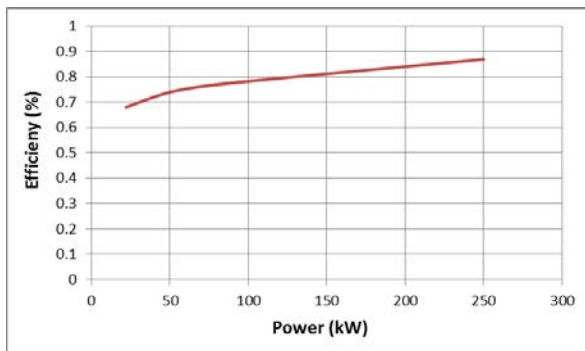
FIGURE 16: MEASURED MECHANICAL TO ELECTRICAL PTO EFFICIENCY
