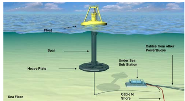
FIGURE 1: EXAMPLE OF OPT POWERBUOY SYSTEM
