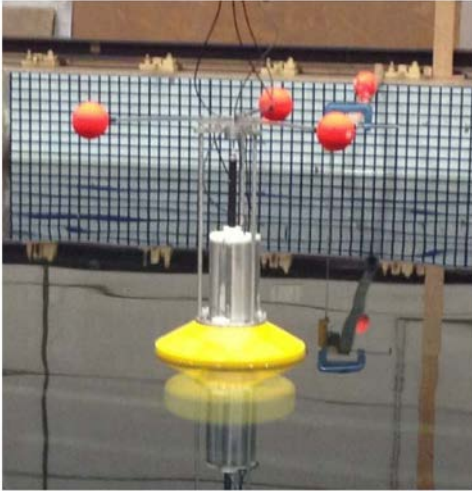
FIGURE 5: EXAMPLE OF OPT REDUCED SCALE MODEL USED IN OPERATIONAL WAVE TANK TESTS [1]. YELLOW FLOAT AND SILVER SPAR ARE VISIBLE ABOVE WATERLINE. RED BALLS ARE USED TO TRACK MOTIONS. BLACK WIRES COMMUNICATE MEASUREMENTS FROM AND CONTROL COMMANDS TO A WORKING PTO INSIDE THE SPAR.
