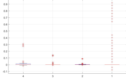
(a) Indegree
