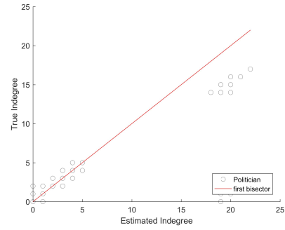
(e) Indegree
