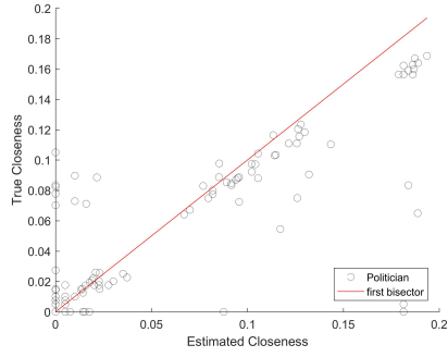
(c) Closeness
