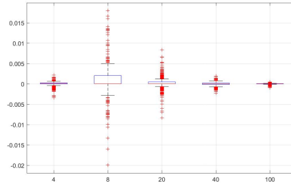
(f) Clustering
