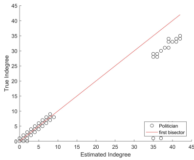
(e) Indegree
