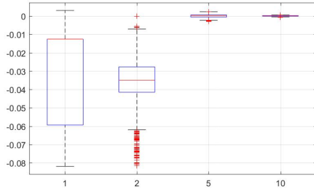
(c) \alpha
