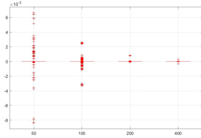
(e) Eigenvector
