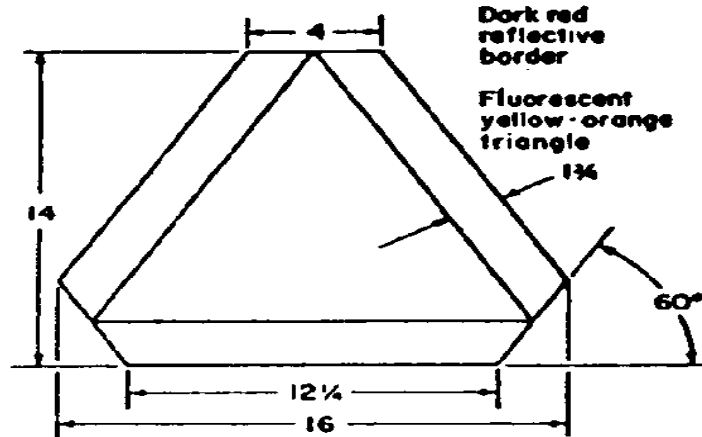
FIGURE J-7.—SLOW-MOVING VEHICLE EMBLEM NOTE: All dimensions are in inches.
