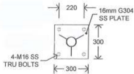
BASE PLATE DETAIL 1:20
