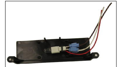
One LED module includes an incandescent light bulb for the license plate light
