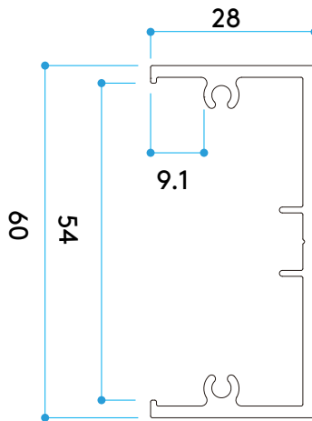
C section
