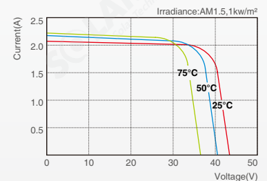
SLP065-24 I-V Curves
