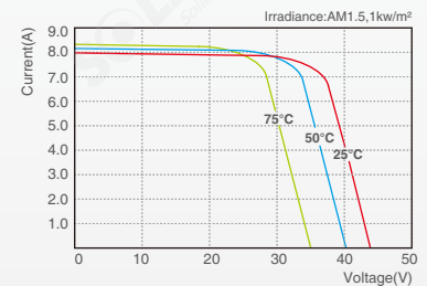
SLP250-24 I-V Curves
