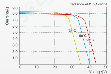
SLP250-24 I-V Curves
