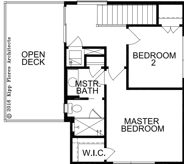
SECOND LEVEL
