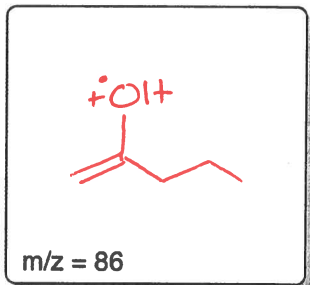
Molecule
