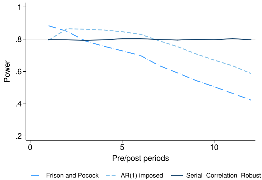
Figure 3: Power simulations for Bloom et al. (2015) data
