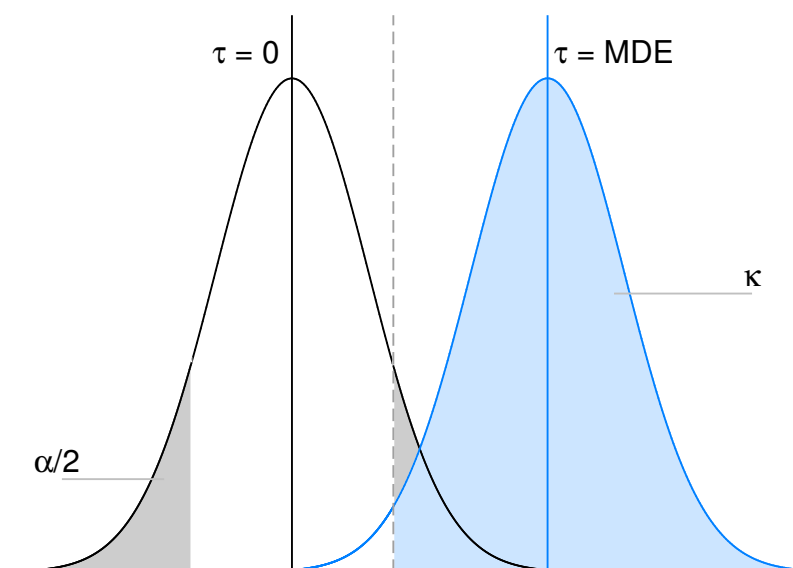
Figure 1: Hypothesis testing framework
