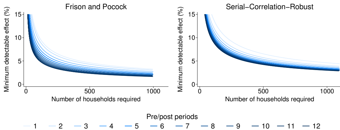
Figure 5: Analytical power calculations – daily Pecan Street dataset
