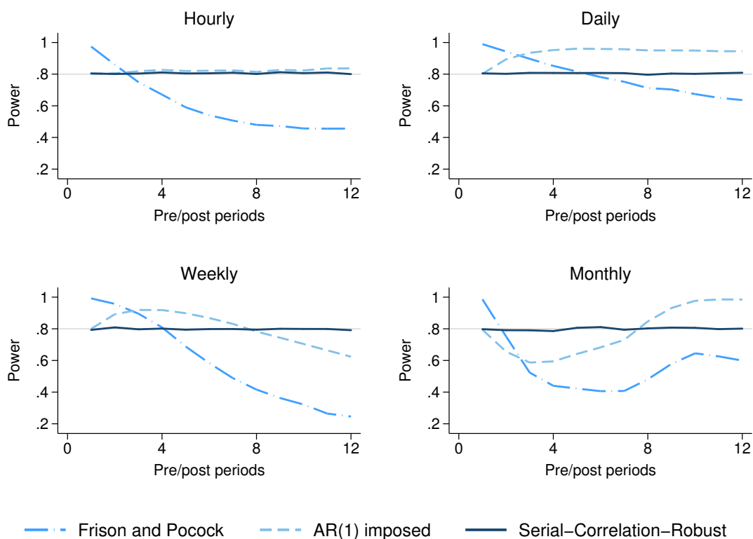
Figure 4: Power simulations for Pecan Street data
