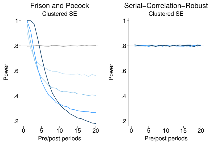
Figure 7: Traditional ANCOVA methods fail under serial correlation
