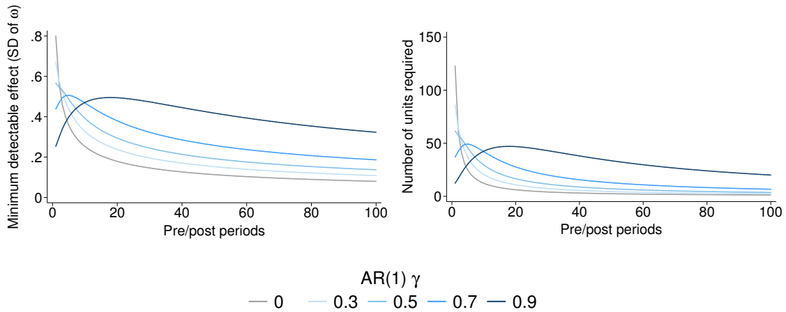
Figure 6: Analytical power calculations with increasing panel length
