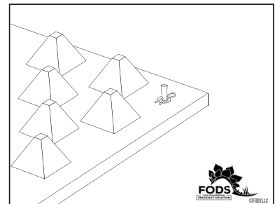
CORNER FORM STAKE ANCHOR SYSTEM
