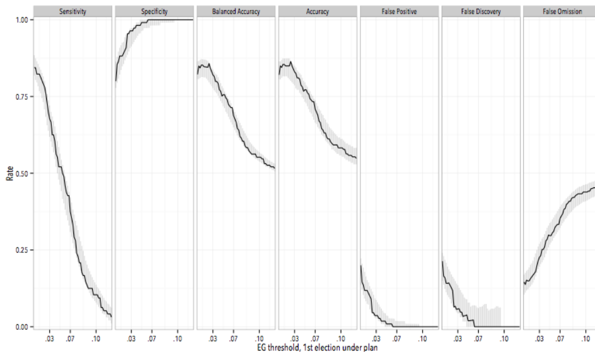
Figure 6: Prognostic performance measures, first efficiency gap under a district plan more extreme than threshold (horizontal axis) as a predictor of whether the average efficiency gap recorded under the district plan has the same sign as the first efficiency gap. Vertical lines indicate 95% confidence intervals. Analysis examines positive, first-election threshold values of the efficiency gap, consistent with Democratic advantage.
