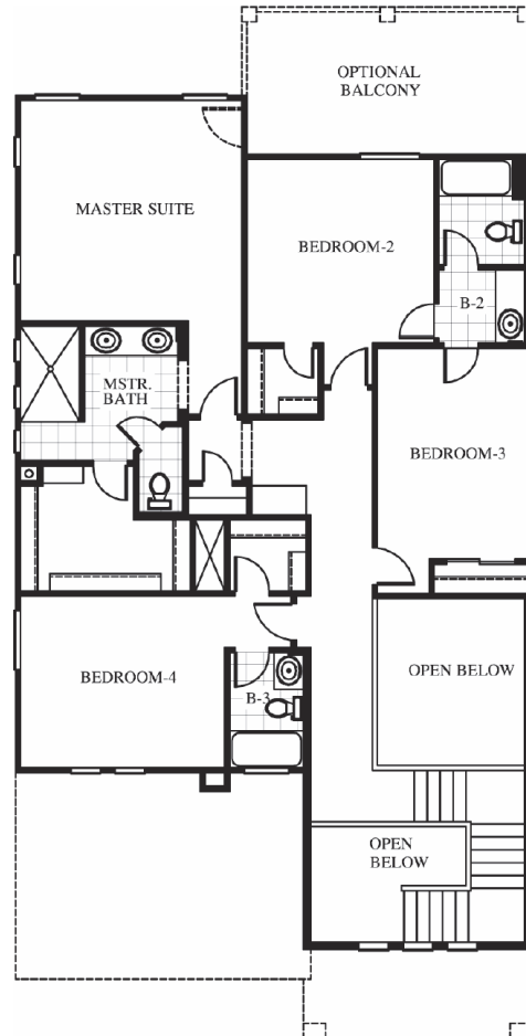
SECOND FLOOR
