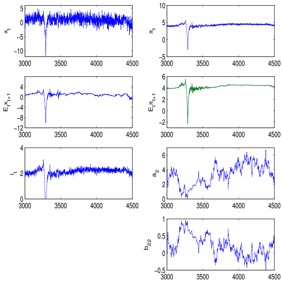
Figure 13: Inflation dynamics in NK Model with a 4% target and a zero lower bound.
