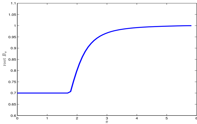
Figure 9: Random-walk beliefs for various inflation targets. Figure plots the largest root of agents' VAR matrix B in the New Keynesian model with the baseline calibration.
