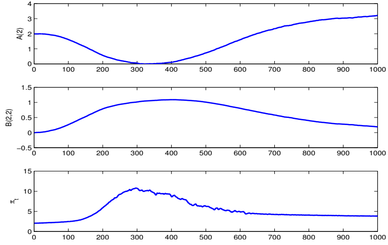
Figure 10: Increasing the Inflation target from 2% to 4%.
