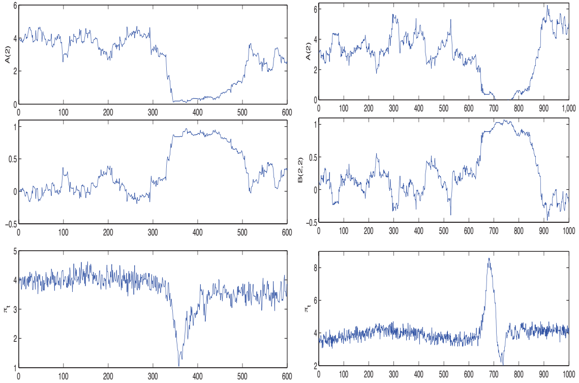
Figure 11: Inflation dynamics in NK Model with a 4% target.
