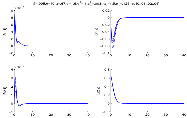
Figure 14: Policy target communication.
