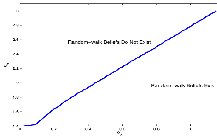
Figure 12: A Policy Frontier for Random-walk beliefs. All pairs of policy coefficients (\alpha_x, \alpha_\pi) below the line can lead to random-walk beliefs in the mean dynamics for the NK model with the baseline calibration, and policy coefficients above the line do not exhibit random-walk beliefs.
