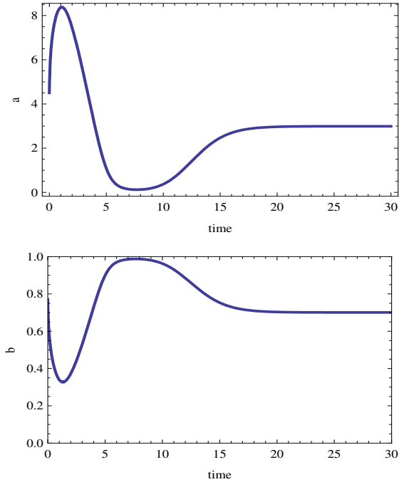
Figure 17: Mean dynamics in NK Model with a price-level targeting rule.
