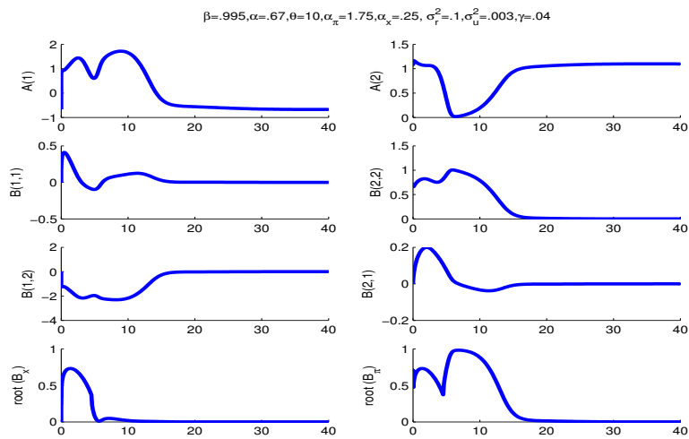
Figure 7: Mean dynamics in NK Model with a 4% target.
