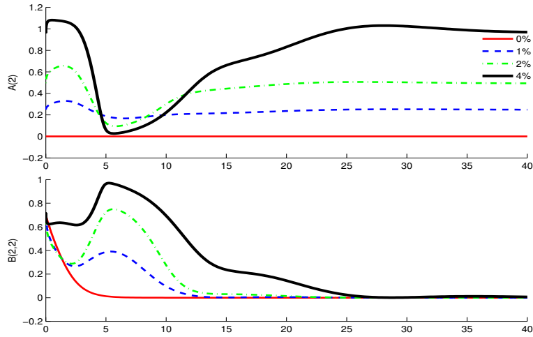
Figure 8: Mean dynamics in NK Model with alternative inflation targets.
