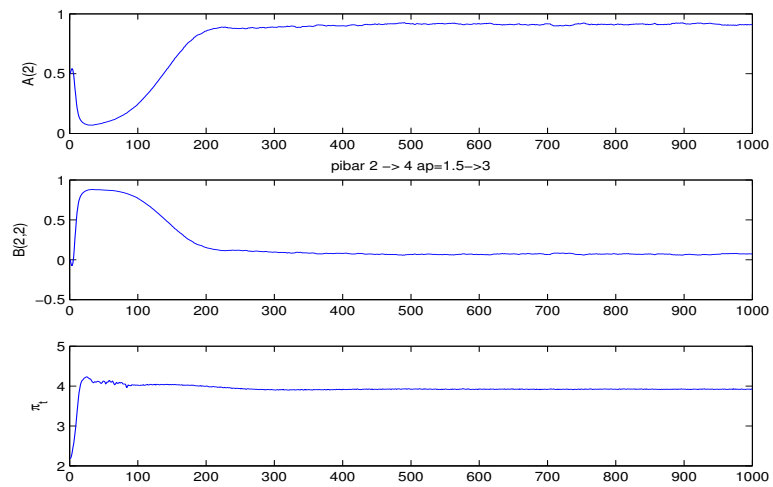
Figure 15: Increasing the target from 2% to 4% and increasing \alpha_\pi from 1.5 to 3.0.
