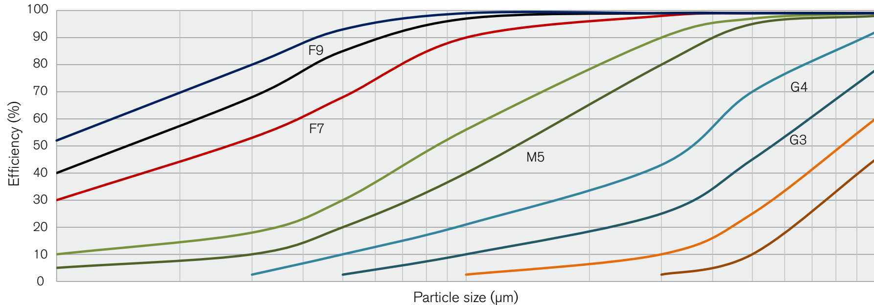
Particle Size Efficiency Chart
