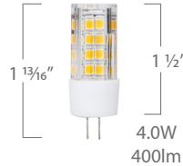
EA-G4-4.0W-001-2780 EA-G4-4.0W-001-3080
