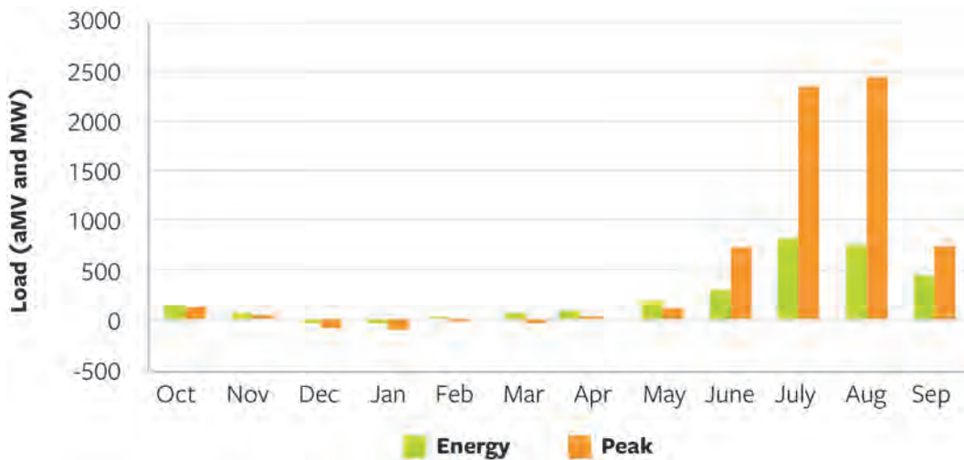
Figure 12. Projected Changes in 2035 Average and Peak Loads (NWPC 2015)
