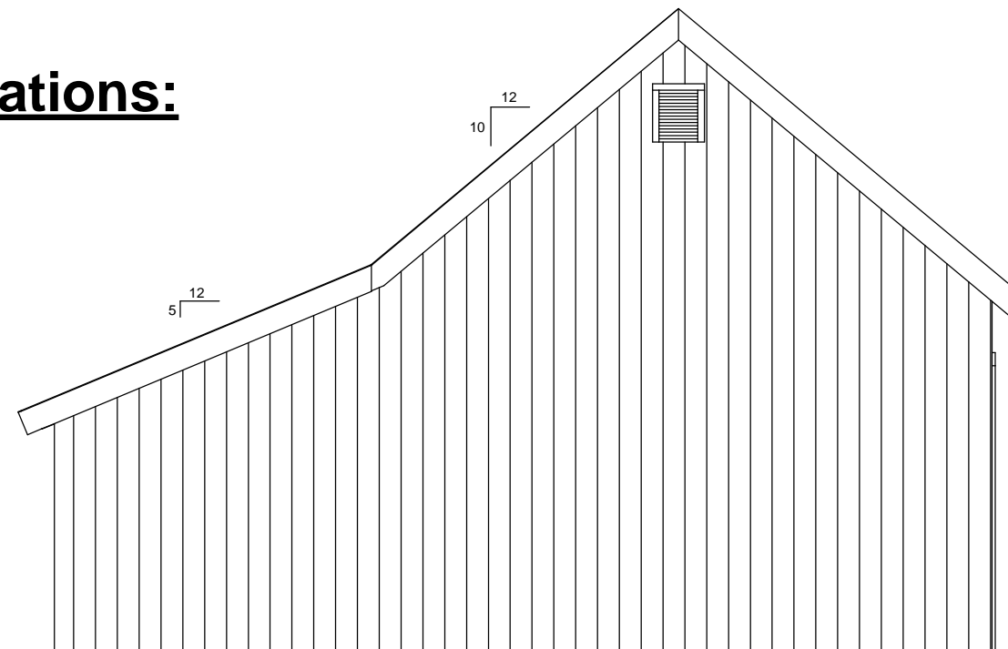
Left Elevation
